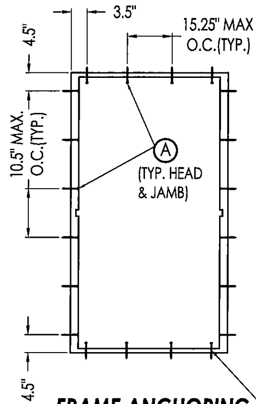
FRAME ANCHORING
