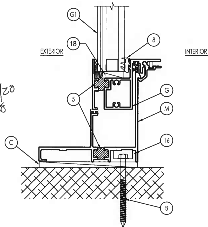
3 3 VERTICAL CROSS SECTION
