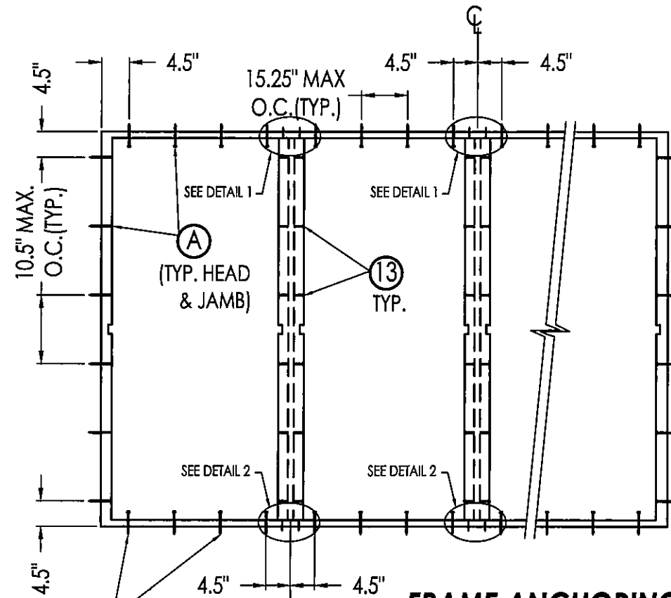
FRAME ANCHORING
