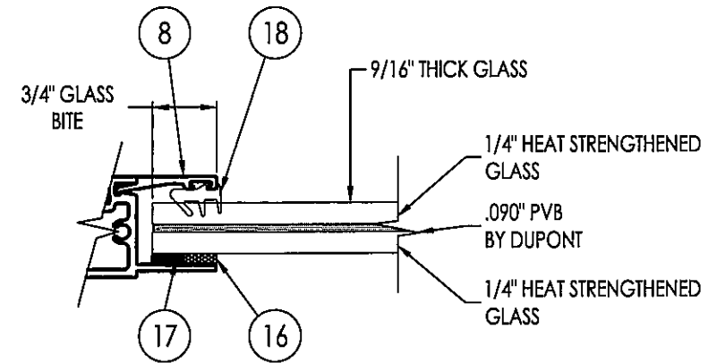
G4 GLAZING DETAIL
