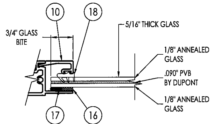
G3 GLAZING DETAIL
