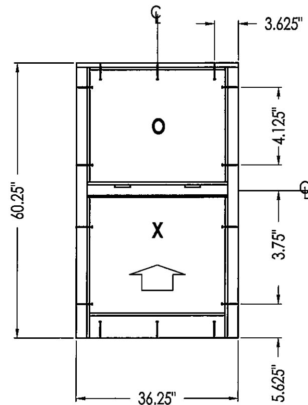
FRAME ANCHORING FOR DP UP TO & INCLUDING +80 / -85 PSF.
