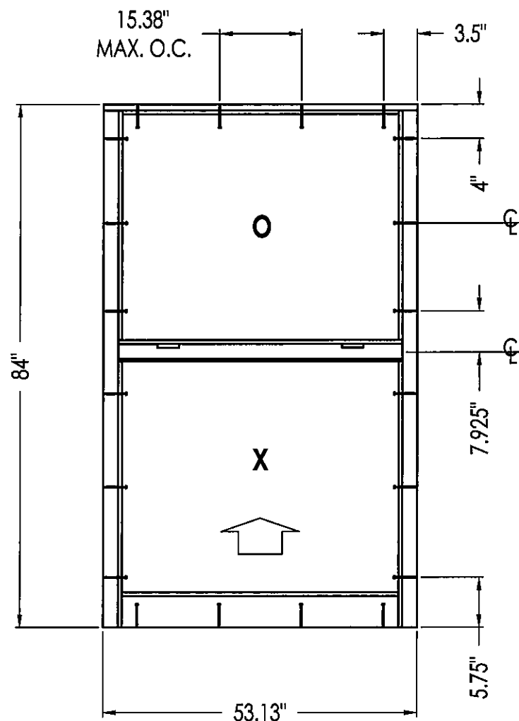
FRAME ANCHORING FOR DP UP TO & INCLUDING +60 / -65 PSF.
