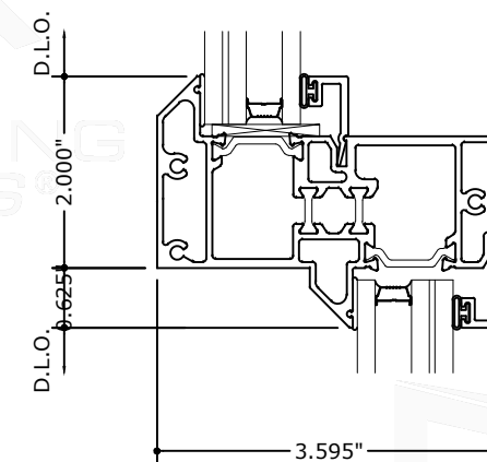
5 INTERMEDIATE HORIZONTAL DETAIL
