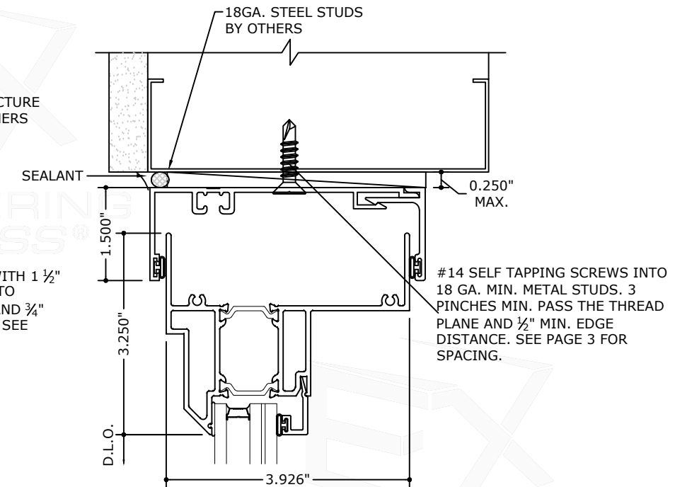
1.5 HEAD DETAIL
