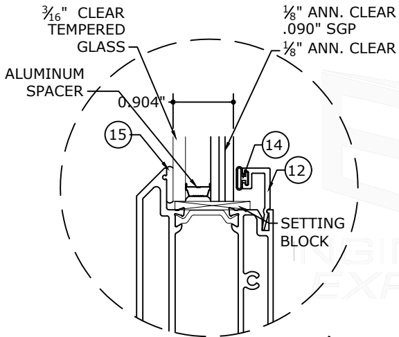
GLASS TYPE G1 GLAZING DETAIL N.T.S.
