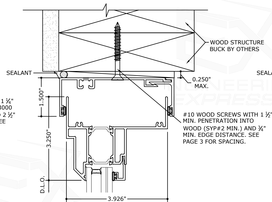
1.4 HEAD DETAIL
