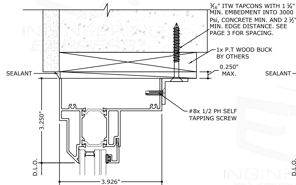
1 HEAD DETAIL
