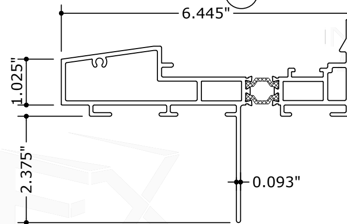
6 HEAD/JAMB RECEPTOR
