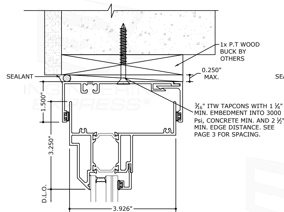
1.3 HEAD DETAIL
