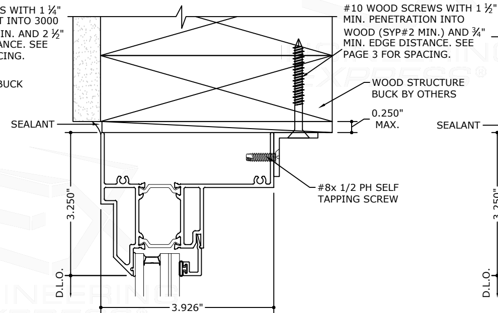
1.1 HEAD DETAIL
