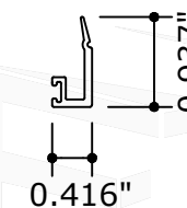
12 GLAZING BEAD
