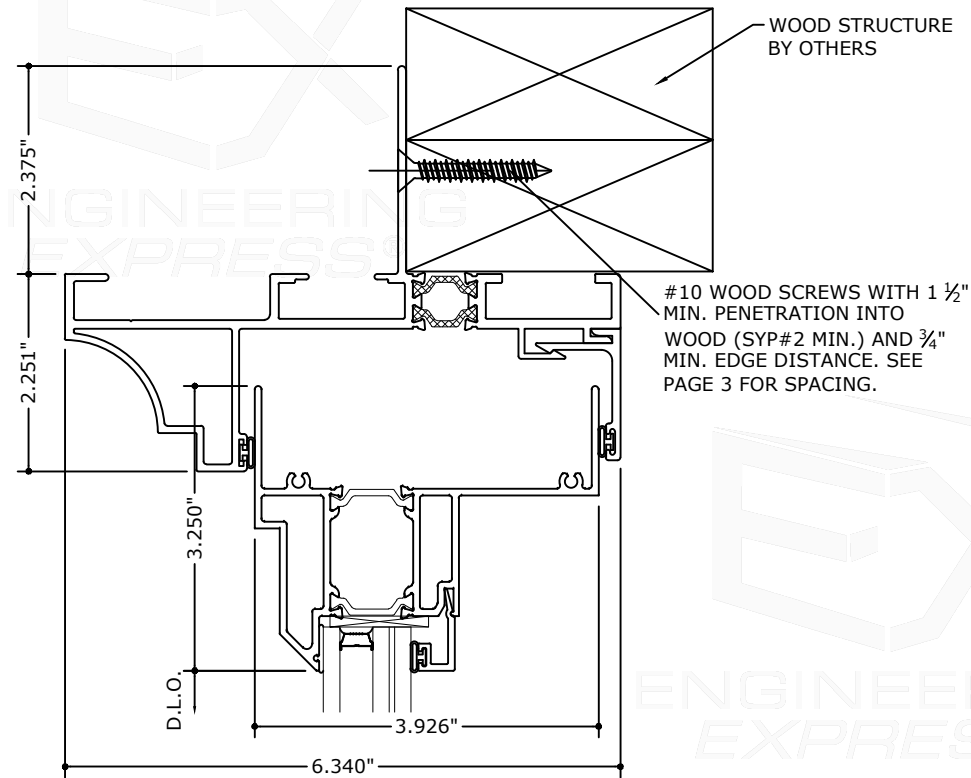
3 HEAD DETAIL
