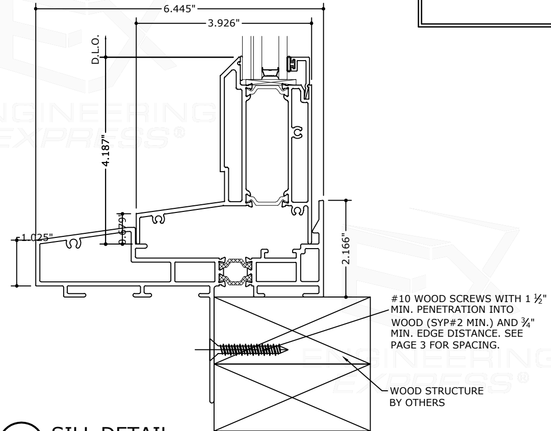
4 SILL DETAIL
