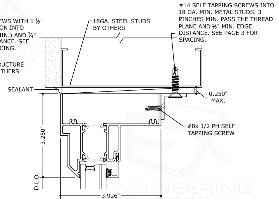
1.2 HEAD DETAIL
