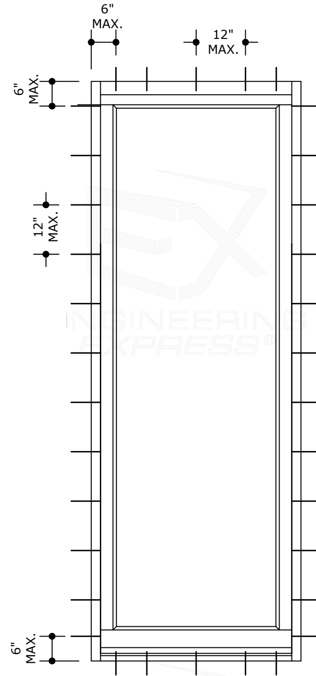
SINGLE LITE ELEVATION
