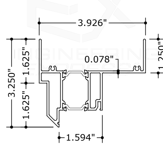
1 FRAME HEAD
