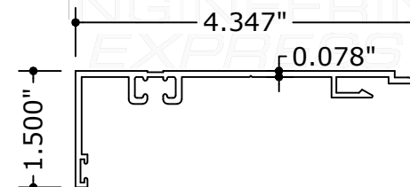
2 FRAME SILL
