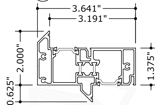
5 HORIZONTAL INTERMEDIATE
