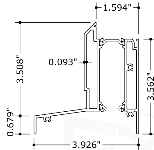
2 FRAME SILL
