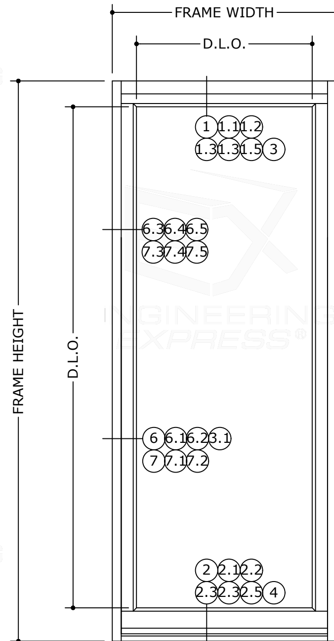
SINGLE LITE ELEVATION
