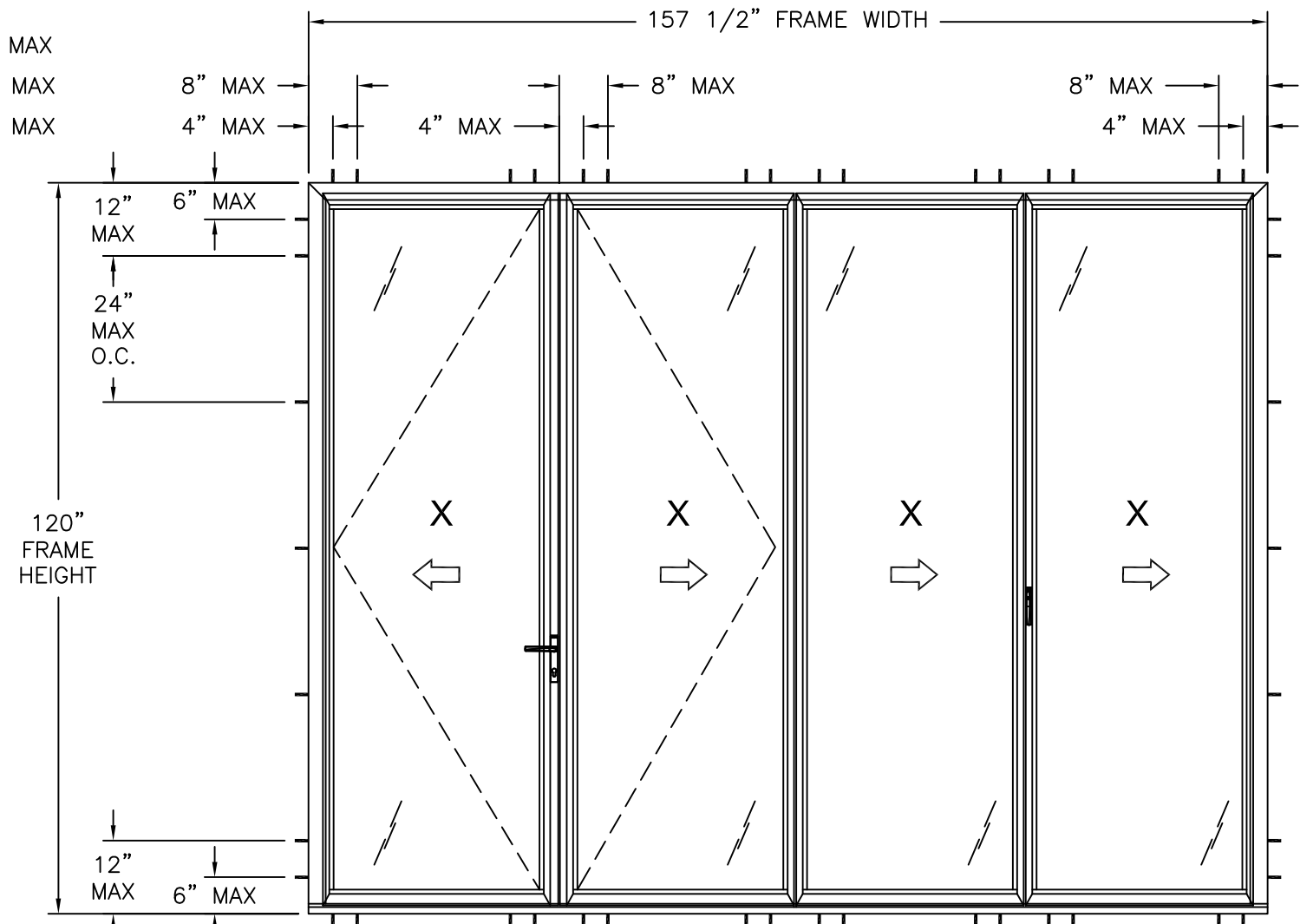
SL70 OUTSWING FOLDING PANEL SYSTEM ANCHORING LAYOUT FOR UNITS LOWER THAN 40PSF
