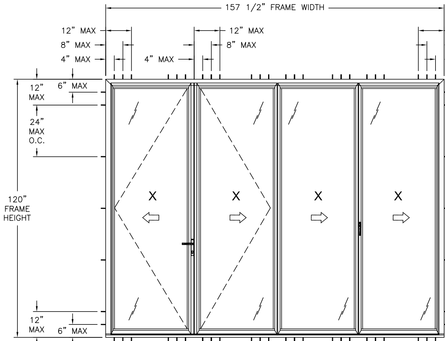
SL70 OUTSWING FOLDING PANEL SYSTEM ANCHORING LAYOUT FOR UNITS HIGHER THAN 40PSF
