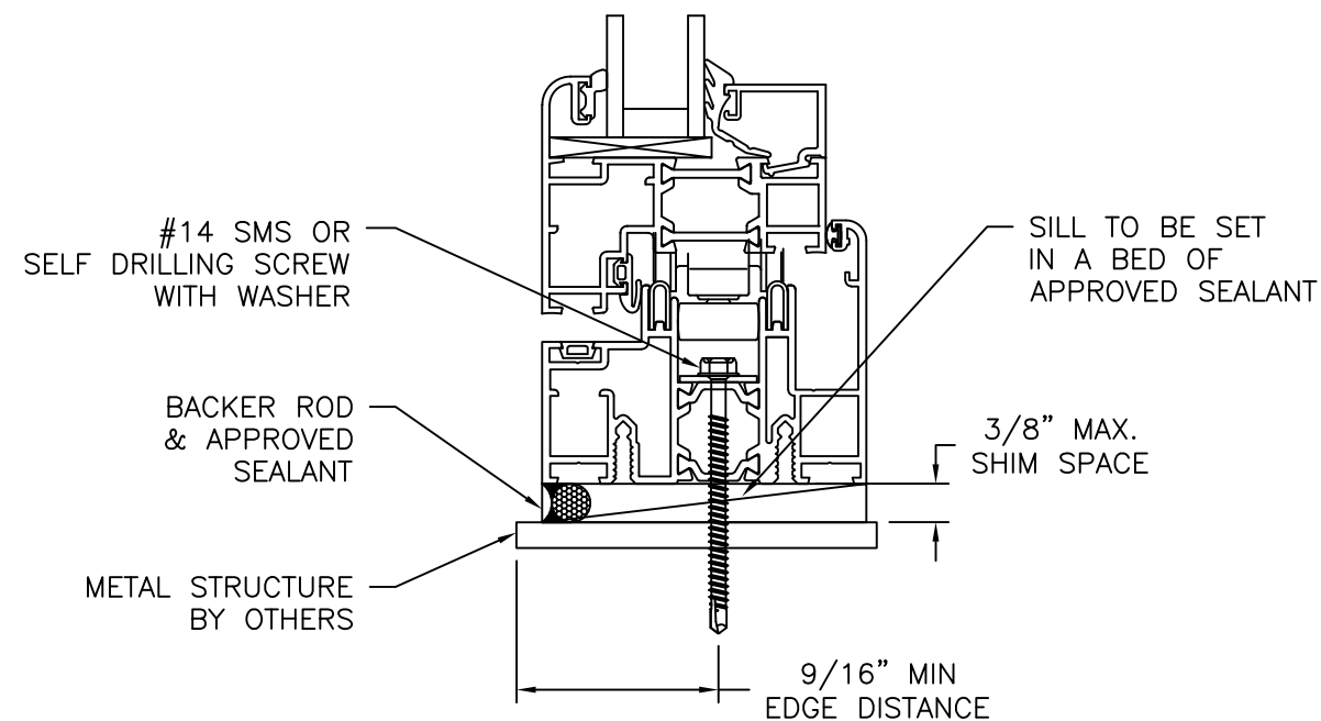
VERTICAL CROSS SECTION METAL STRUCTURE INSTALLATION HIGH PERFORMANCE SILL SHOWN, OTHER SILLS SIMILAR
