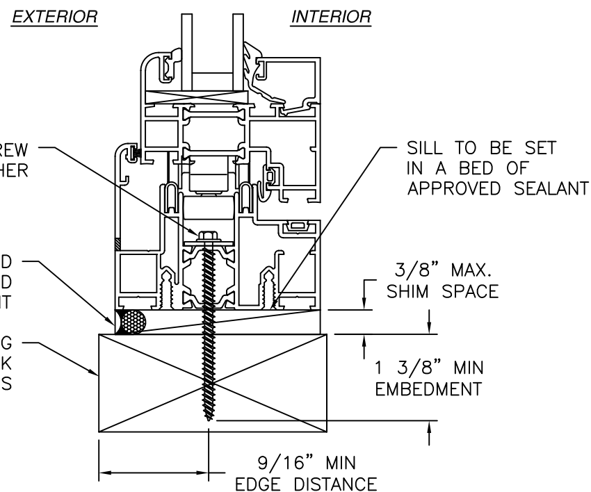
VERTICAL CROSS SECTION WOOD FRAMING OR 2X BUCK INSTALLATION HIGH PERFORMANCE SILL SHOWN, OTHER SILLS SIMILAR
