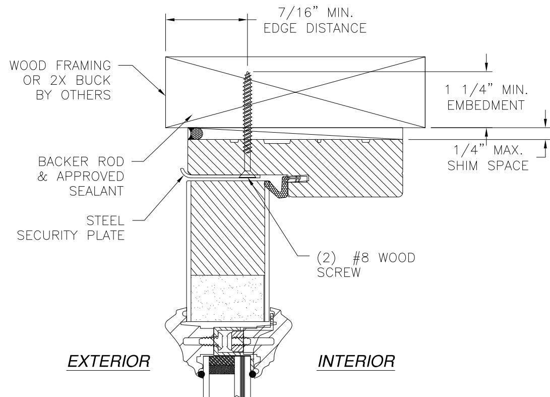
KEEPER INSTALLATION DETAIL WOOD FRAMING OR 2X BUCK INSTALLATION
