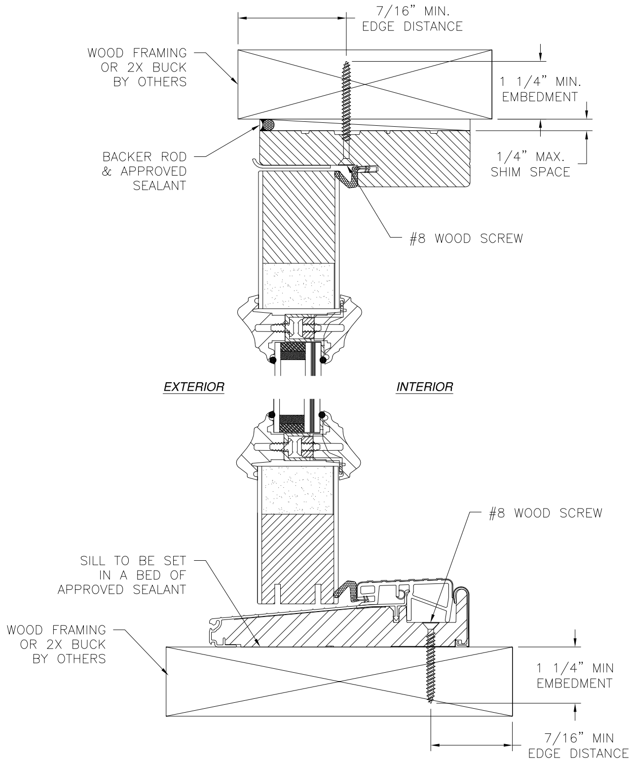
VERTICAL CROSS SECTION DOOR INSTALLATION WOOD FRAMING OR 2X BUCK INSTALLATION
