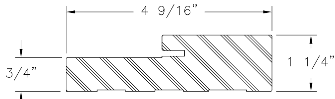
COMPOSITE FRAME PROFILE
