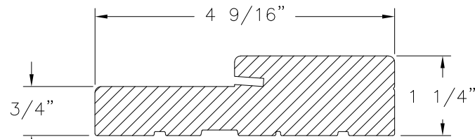
WOOD FRAME PROFILE
