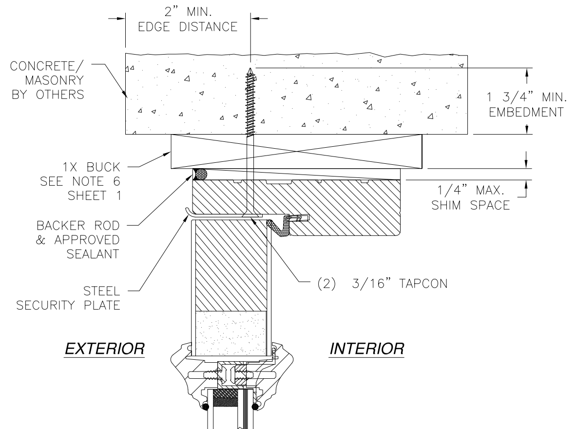
KEEPER INSTALLATION DETAIL CONCRETE/MASONRY INSTALLATION
