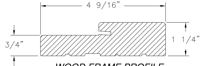
WOOD FRAME PROFILE
