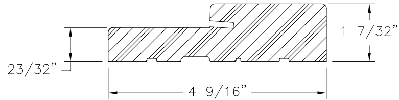
FRAMESAVER COMPOSITE
