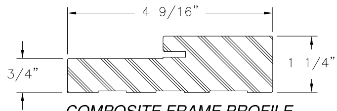
COMPOSITE FRAME PROFILE
