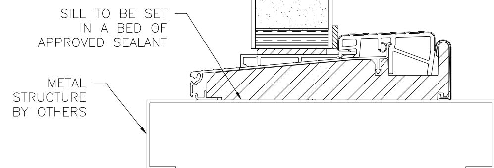
VERTICAL CROSS SECTION STANDARD SIDELITE INSTALLATION METAL STRUCTURE INSTALLATION
