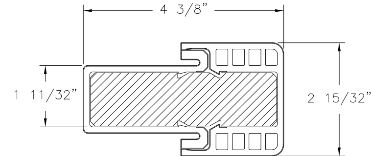
HYBRID FAT BOY MULLION COMPOSITE
