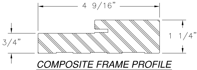
WOOD FRAME PROFILE
