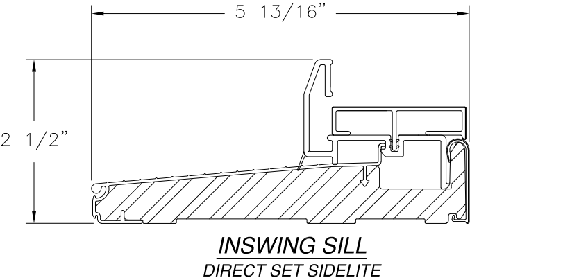
INSWING SILL STANDARD SIDELITE
