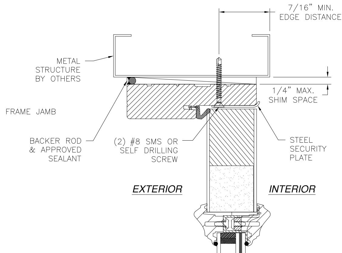
KEEPER INSTALLATION DETAIL METAL STRUCTURE INSTALLATION
