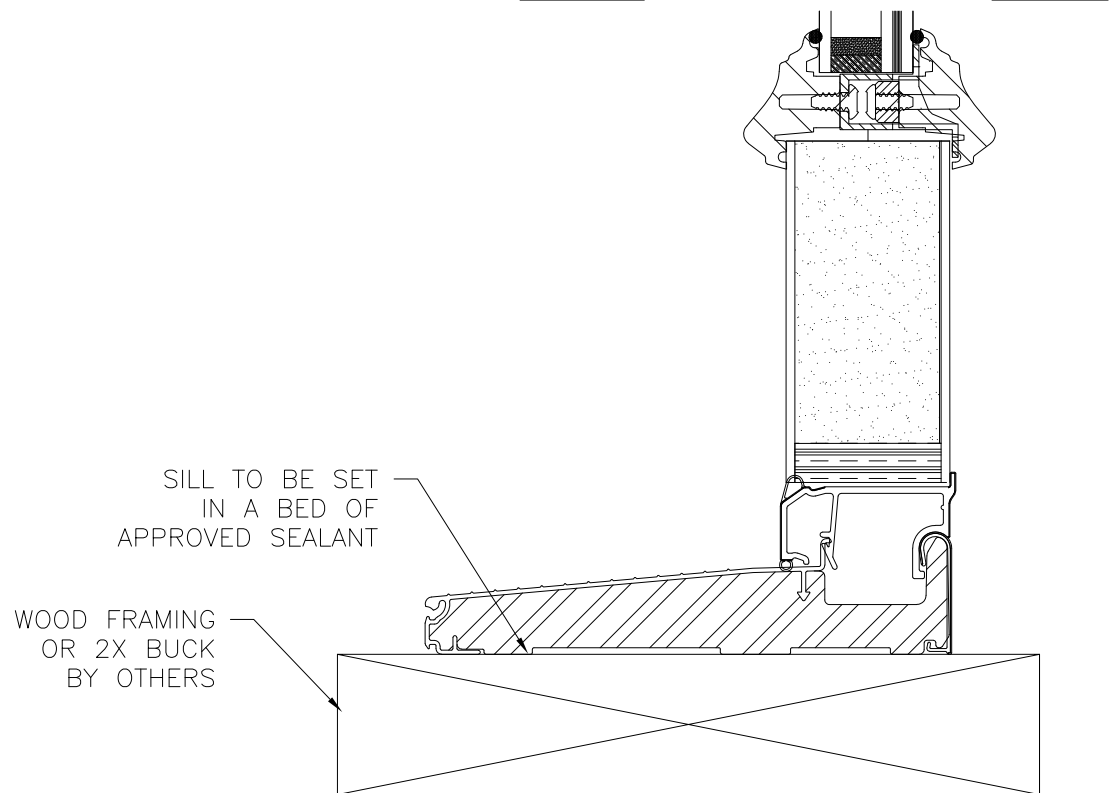
VERTICAL CROSS SECTION STANDARD SIDELITE INSTALLATION WOOD FRAMING OR 2X BUCK INSTALLATION
