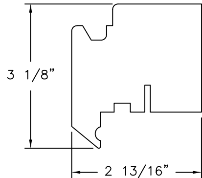
— SASH TOP RAIL (FRENCH OAK)
