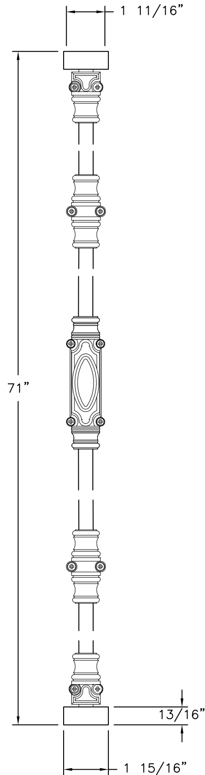
CREMONE TYPE RG 50 FROM REMY GARNIER
