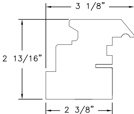
— CASEMENT WINDOW SASH (FRENCH OAK)
