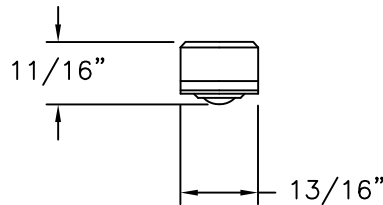
— METALLIC BALL FOR SUPPORT (STAINLESS STEEL)
