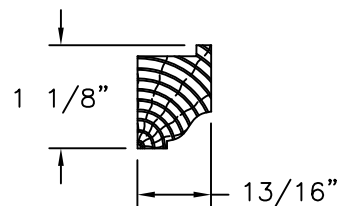
— GLAZING BEAD (FRENCH OAK)
