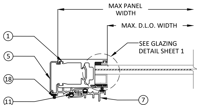
B 6 HORIZONTAL SECTION POCKET WALL
