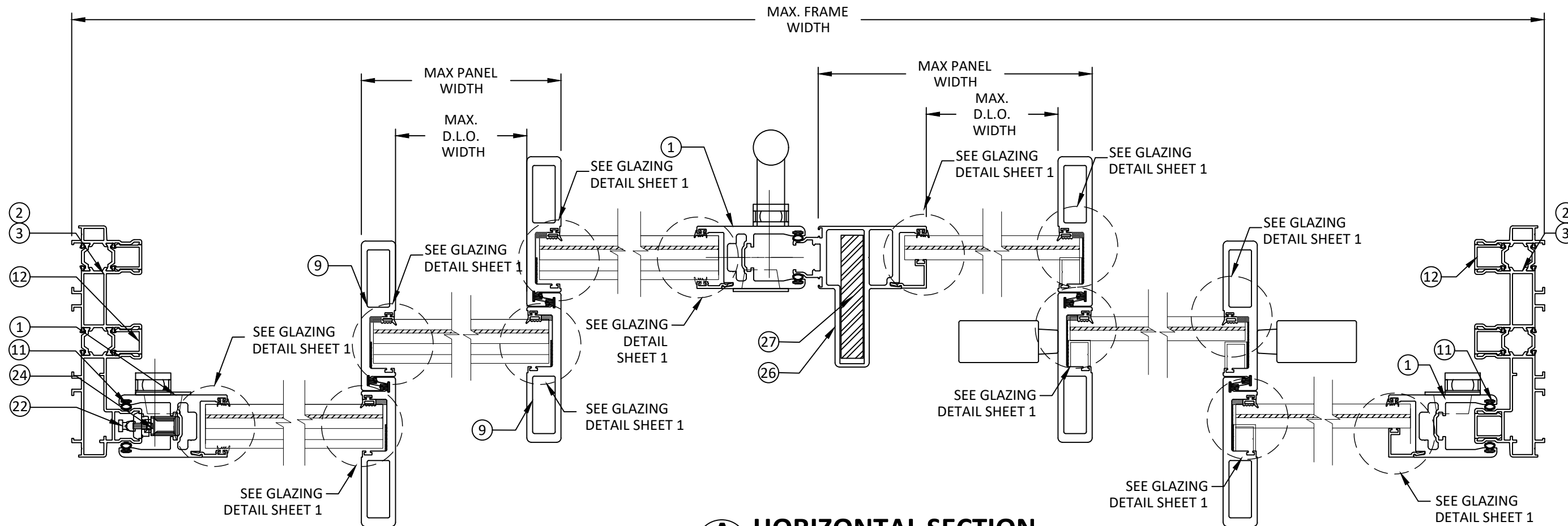
A 6 HORIZONTAL SECTION MEETING STILES 2 OR 3 TRACKS
