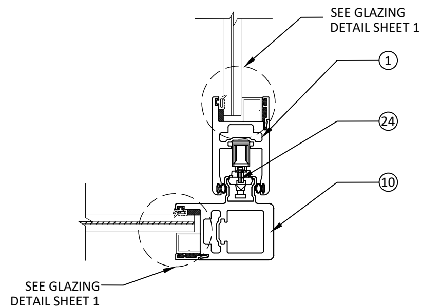
C 6 HORIZONTAL SECTION CORNER DETAIL
