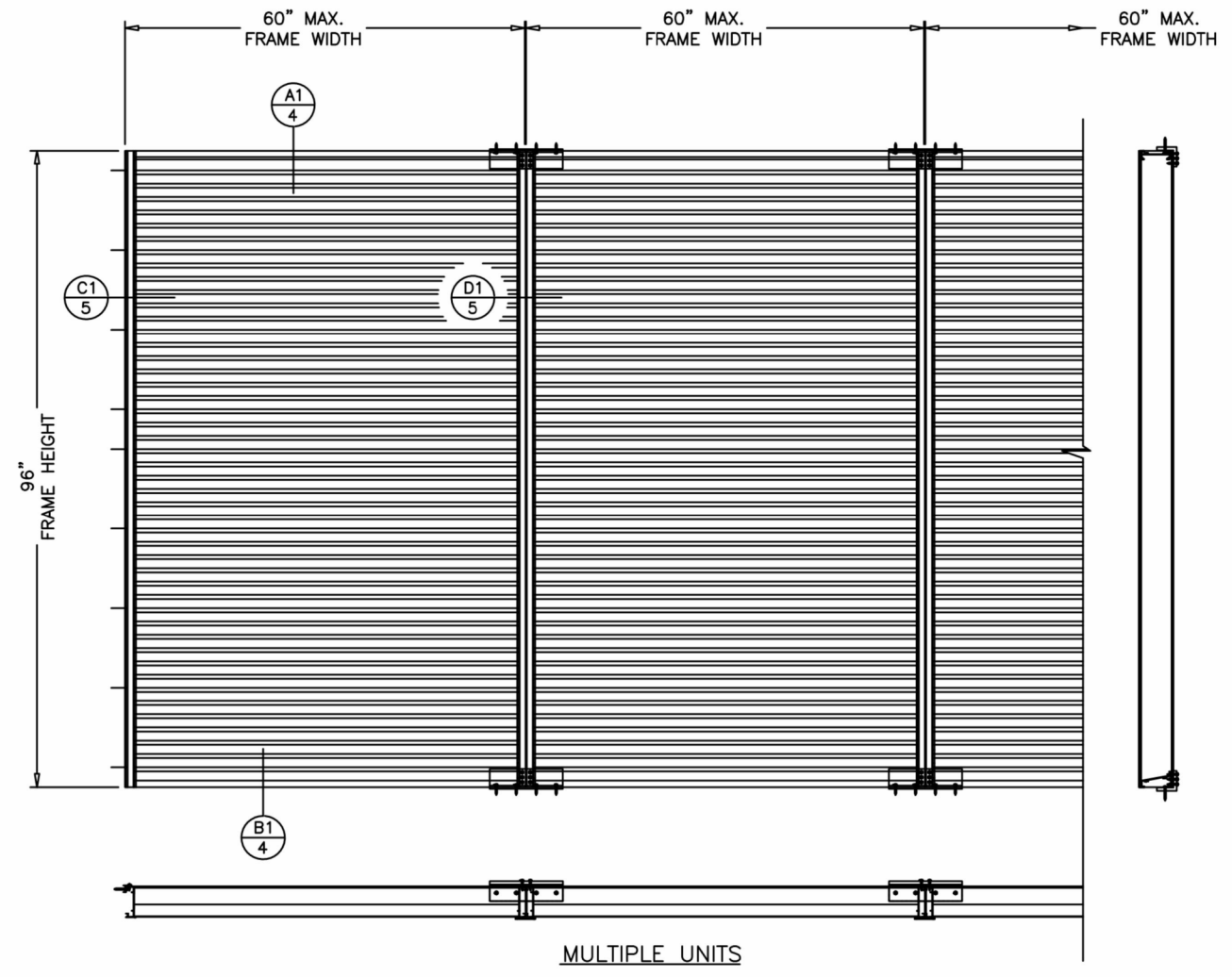
TYPICAL ELEVATIONS
