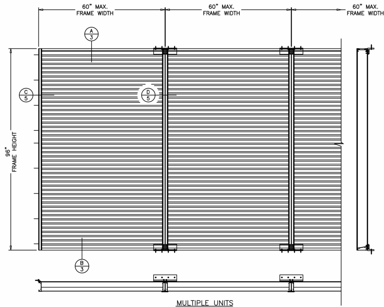
TYPICAL ELEVATIONS
