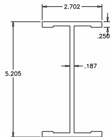
5 SLIP MULLION
