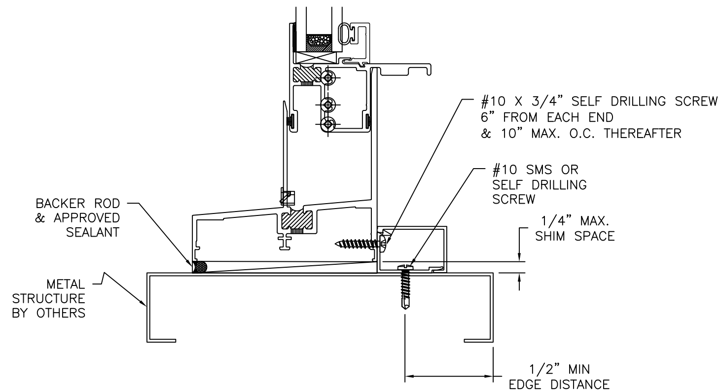
VERTICAL CROSS SECTION METAL STRUCTURE INSTALLATION
