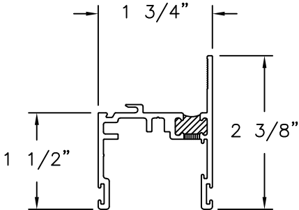
STILE (BAM-1009) ALUMINUM 6063-T6
