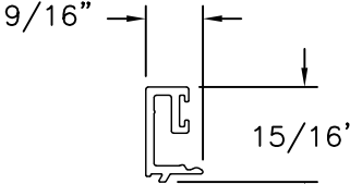
GLAZING BEAD (BAM-1020) ALUMINUM 6063-T6
