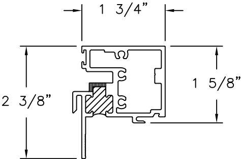
LOCK RAIL (BAM-1007) ALUMINUM 6063-T6
