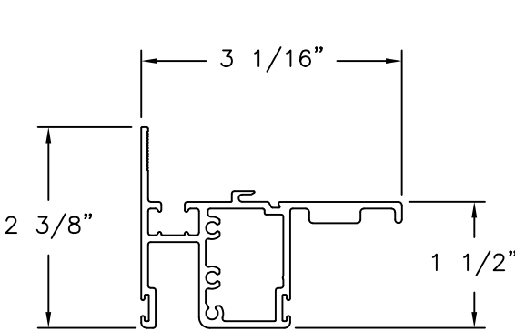
BOTTOM RAIL (BAM-1008) ALUMINUM 6063-T6
