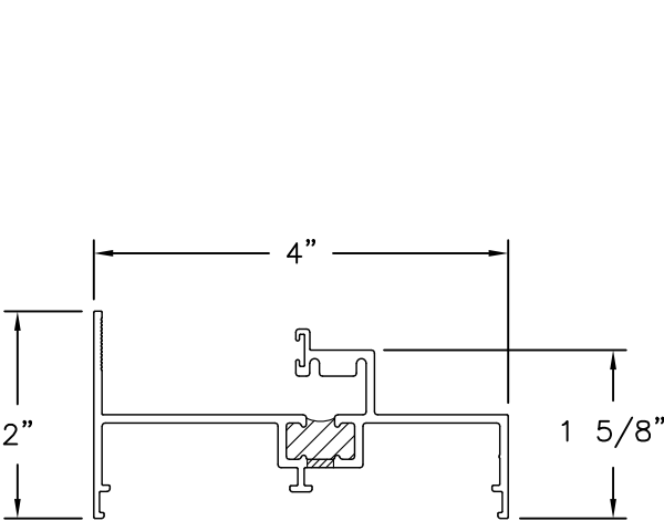
HEAD (BAM-1000) ALUMINUM 6063-T6
