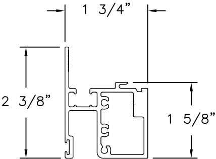
TOP RAIL (BAM-1005) ALUMINUM 6063-T6
