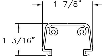
SASH STOP (BAM-1018) ALUMINUM 6063-T6
