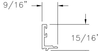
GLAZING BEAD (BAM-1015) ALUMINUM 6063-T6
