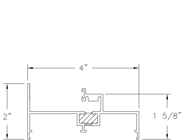
HEAD (BAM-1000) ALUMINUM 6063-T6
