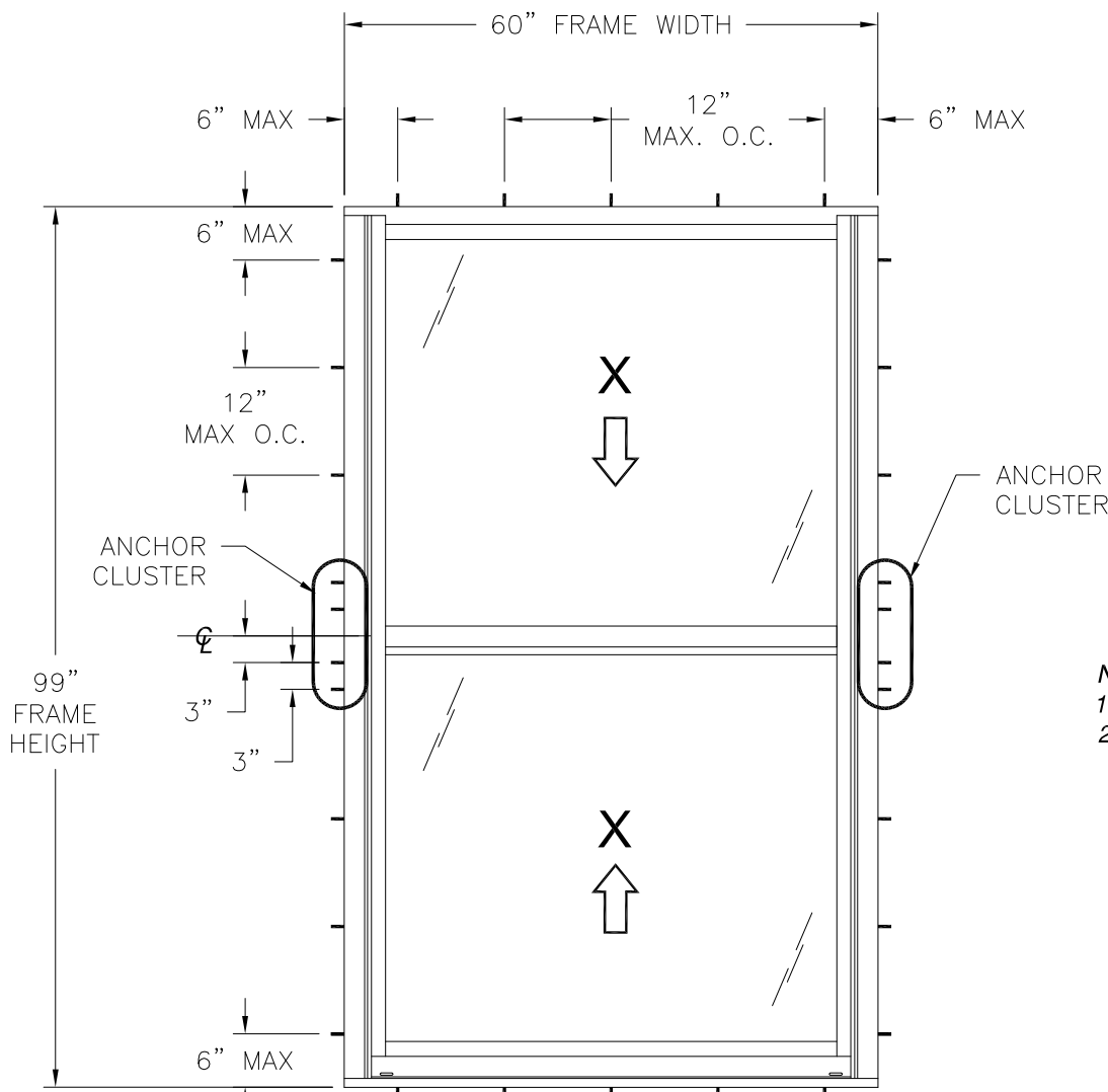
3500 SERIES DOUBLE HUNG WINDOW - IMPACT EXTERIOR VIEW
