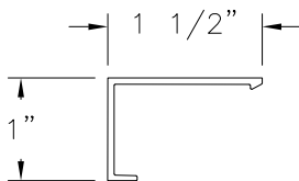
TRIM COVER (WLB-2004) ALUMINUM 6063-T5
