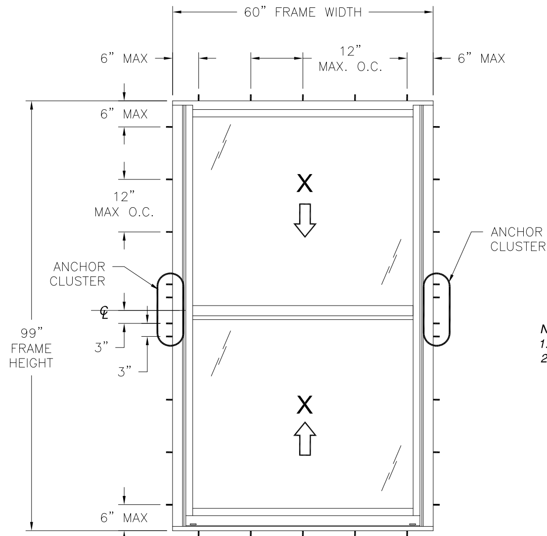
3500 SERIES DOUBLE HUNG WINDOW NON-IMPACT EXTERIOR VIEW
