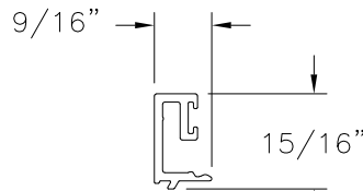
GLAZING BEAD (BAM-1020) ALUMINUM 6063-T6
