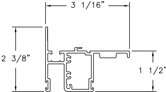
BOTTOM RAIL (BAM-1008) ALUMINUM 6063-T6
