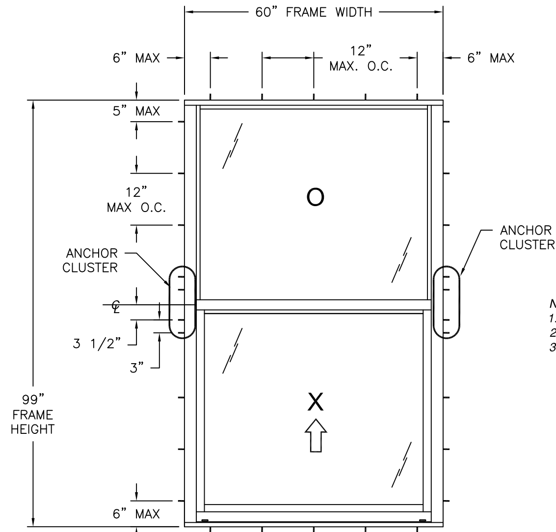
3000 SERIES SINGLE HUNG WINDOW NON-IMPACT EXTERIOR VIEW
