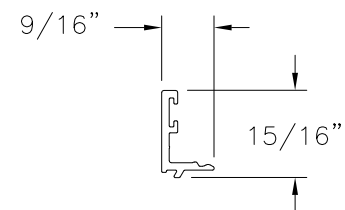
GLAZING BEAD (BAM-1015) ALUMINUM 6063-T6
