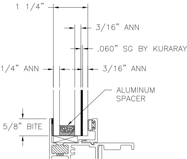
GLAZING DETAIL
