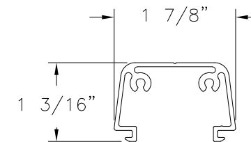
SASH STOP (BAM-1018) ALUMINUM 6063-T6
