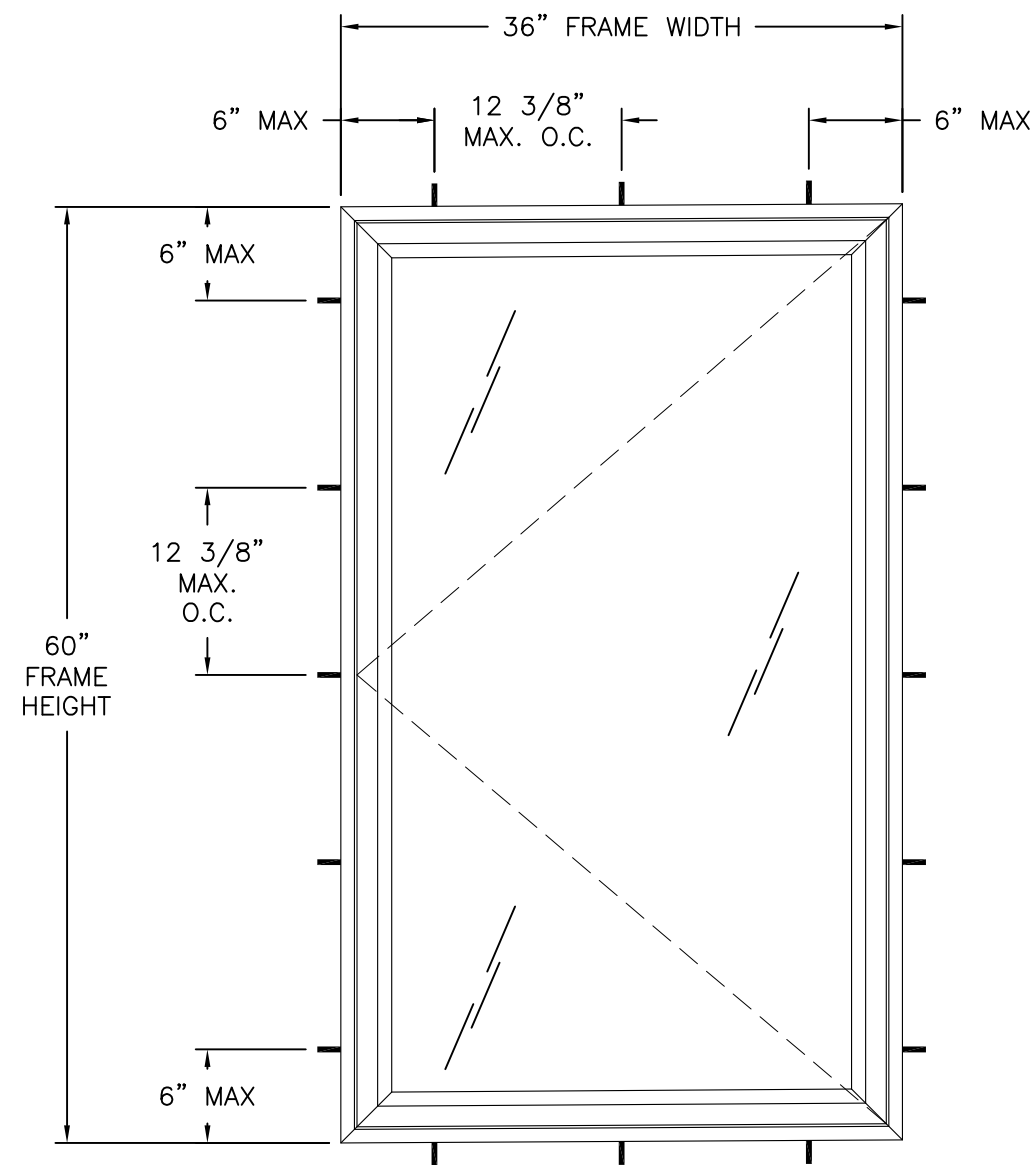
2400 SERIES CASEMENT OUTSWING WINDOW NON-IMPACT EXTERIOR VIEW
