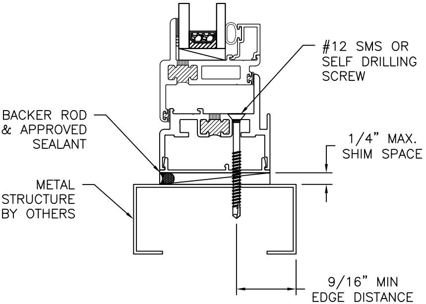
VERTICAL CROSS SECTION METAL STRUCTURE INSTALLATION
