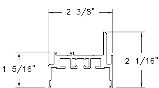
MAIN FRAME (BAM-925) ALUMINUM 6063-T5
