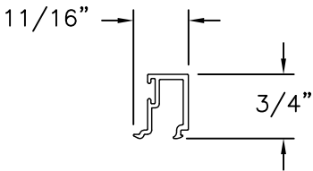
VENT GLAZING BEAD (BAM-922) ALUMINUM 6063-T5
