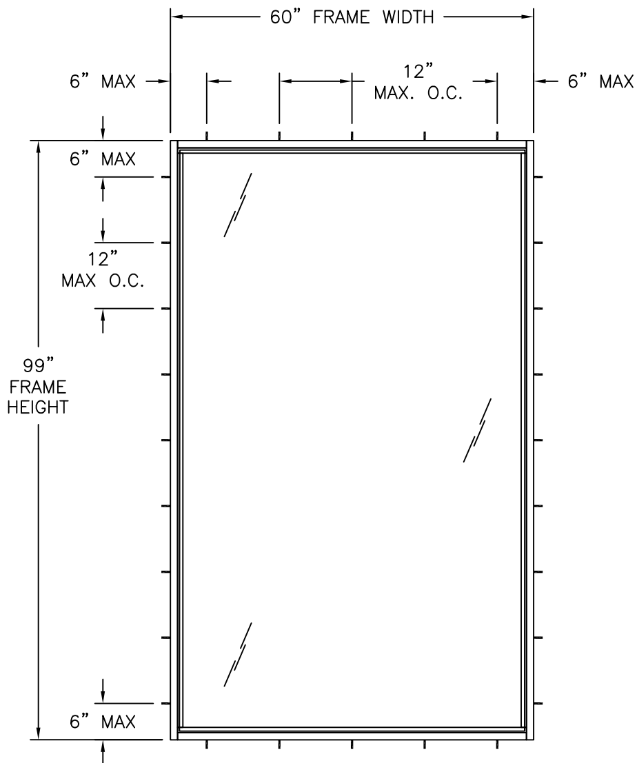
4000 SERIES FIXED WINDOW - IMPACT EXTERIOR VIEW
