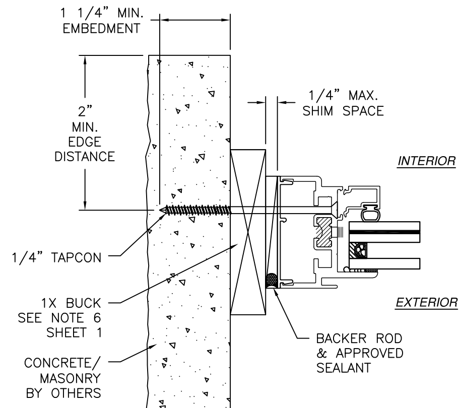
JAMB INSTALLATION DETAIL FIXED WINDOW CONCRETE/MASONRY WITH 1X BUCK INSTALLATION FOR INSTALLATION WITHOUT 1X BUCK REFER TO JAMB INSTALLATION DETAIL SHEET 5
