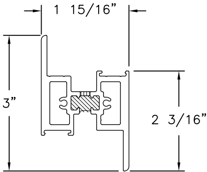
INTERMEDIATE BOTTOM (BAM-905) ALUMINUM 6063-T6
