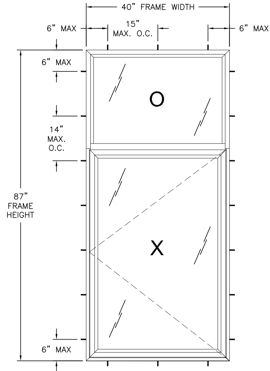
2400 SERIES FIXED OVER CASEMENT OUTSWING WINDOW NON-IMPACT EXTERIOR VIEW
