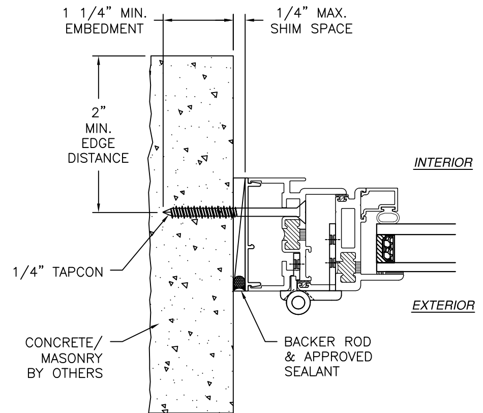
JAMB INSTALLATION DETAIL CONCRETE/MASONRY WITHOUT 1X BUCK INSTALLATION FOR CONCRETE/MASONRY INSTALLATION WITH 1X BUCK REFER TO HEAD AND SILL INSTALLATION DETAILS CASEMENT WINDOW SHOWN
