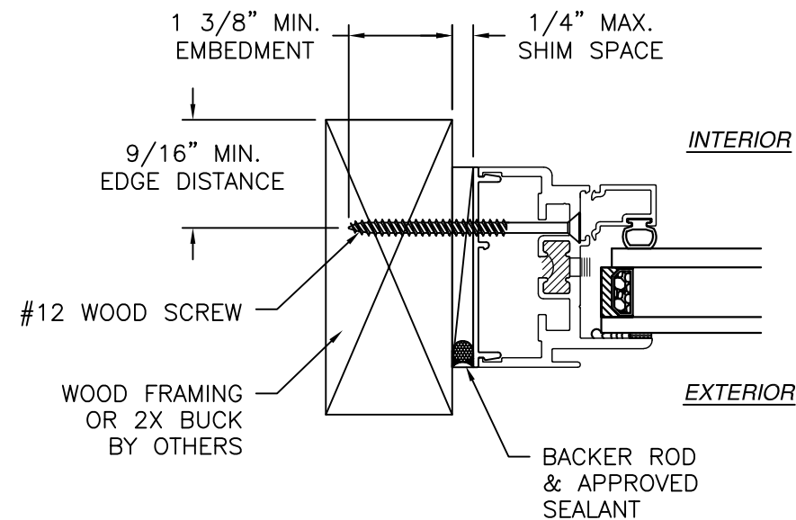
JAMB INSTALLATION DETAIL FIXED WINDOW WOOD FRAMING OR 2X BUCK INSTALLATION
