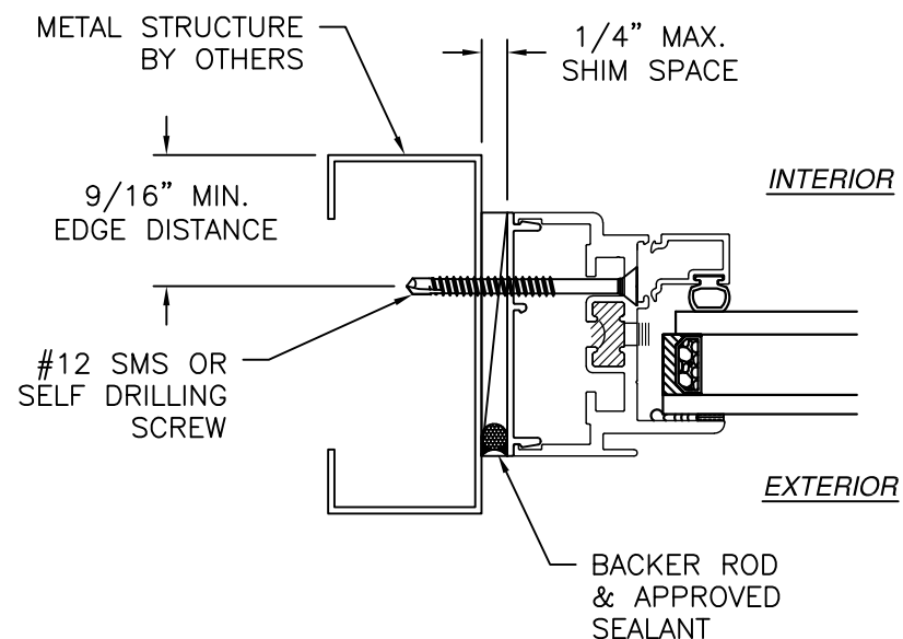
JAMB INSTALLATION DETAIL FIXED WINDOW METAL STRUCTURE INSTALLATION
