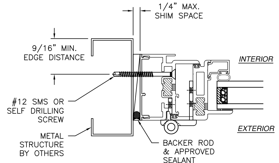
JAMB INSTALLATION DETAIL METAL STRUCTURE INSTALLATION CASEMENT WINDOW SHOWN
