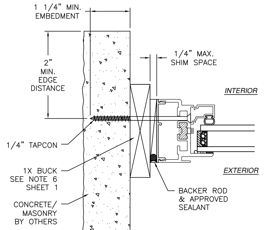
JAMB INSTALLATION DETAIL FIXED WINDOW CONCRETE/MASONRY WITH 1X BUCK INSTALLATION FOR INSTALLATION WITHOUT 1X BUCK REFER TO JAMB INSTALLATION DETAIL SHEET 5
