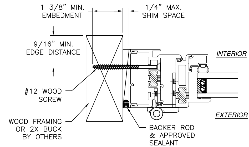
JAMB INSTALLATION DETAIL WOOD FRAMING OR 2X BUCK INSTALLATION CASEMENT WINDOW SHOWN
