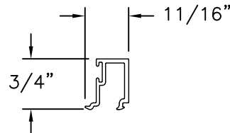
GLAZING BEAD (BAM-922) ALUMINUM 6063-T5
