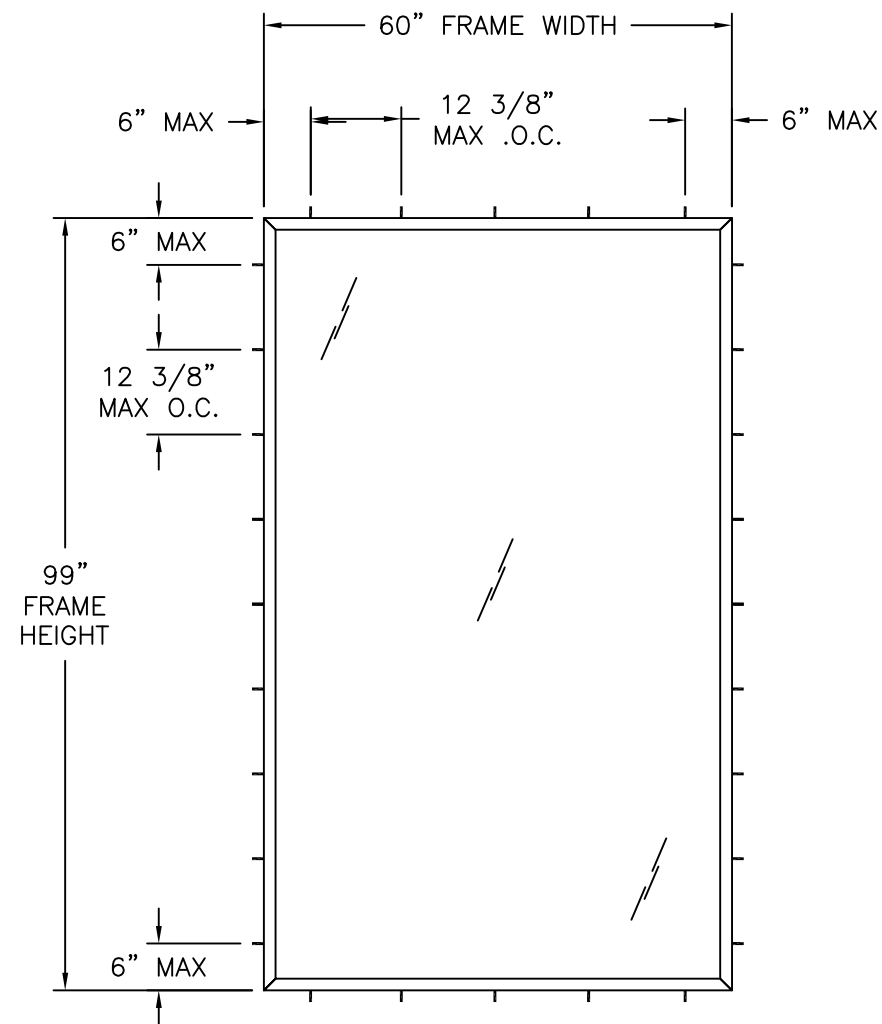
2200 SERIES FIXED WINDOW NON-IMPACT EXTERIOR VIEW
