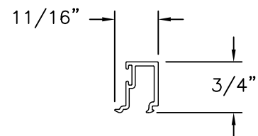
GLAZING BEAD (BAM-922) ALUMINUM 6063-T5
