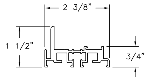
MAIN FRAME (BAM-911) ALUMINUM 6063-T5
