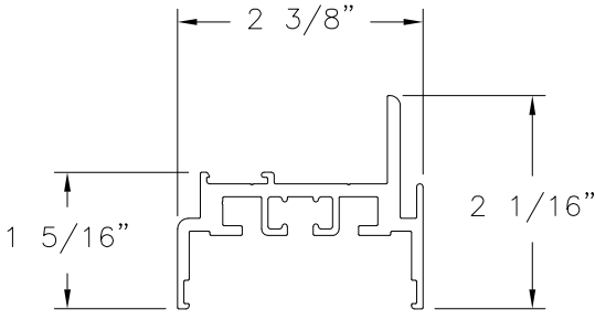
VENT FRAME (BAM-925) ALUMINUM 6063-T5
