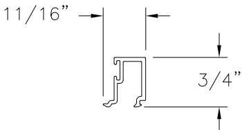
VENT GLAZING BEAD (BAM-922) ALUMINUM 6063-T5
