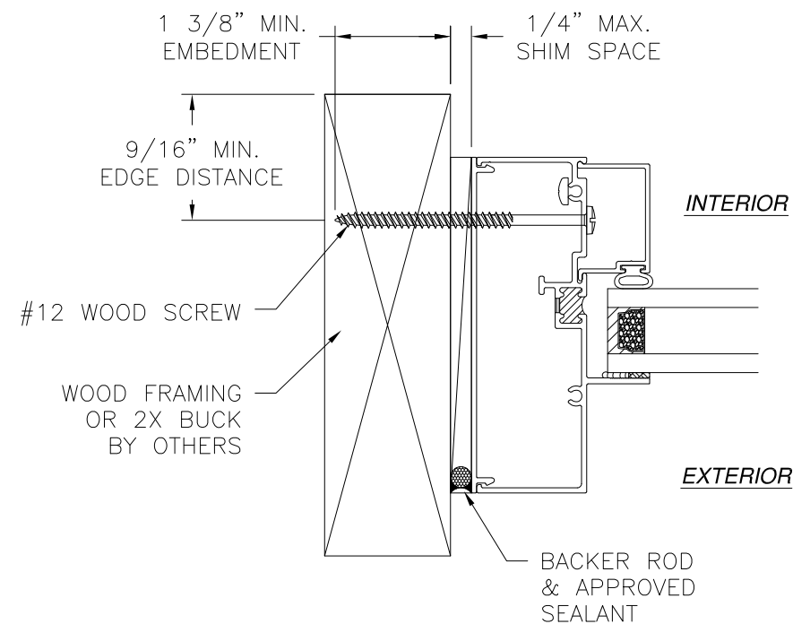
JAMB INSTALLATION DETAIL FIXED WINDOW WOOD FRAMING OR 2X BUCK INSTALLATION
