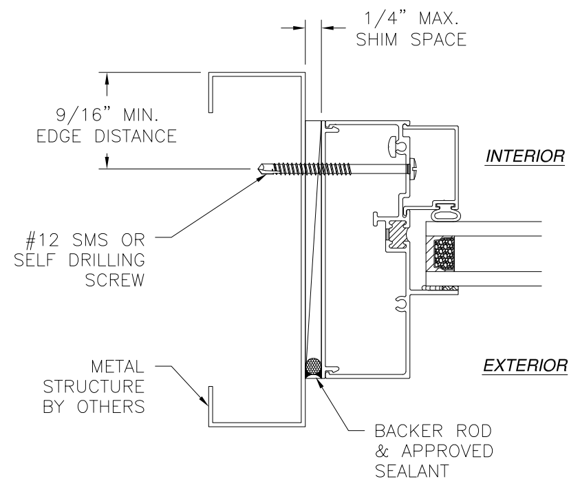
JAMB INSTALLATION DETAIL FIXED WINDOW METAL STRUCTURE INSTALLATION
