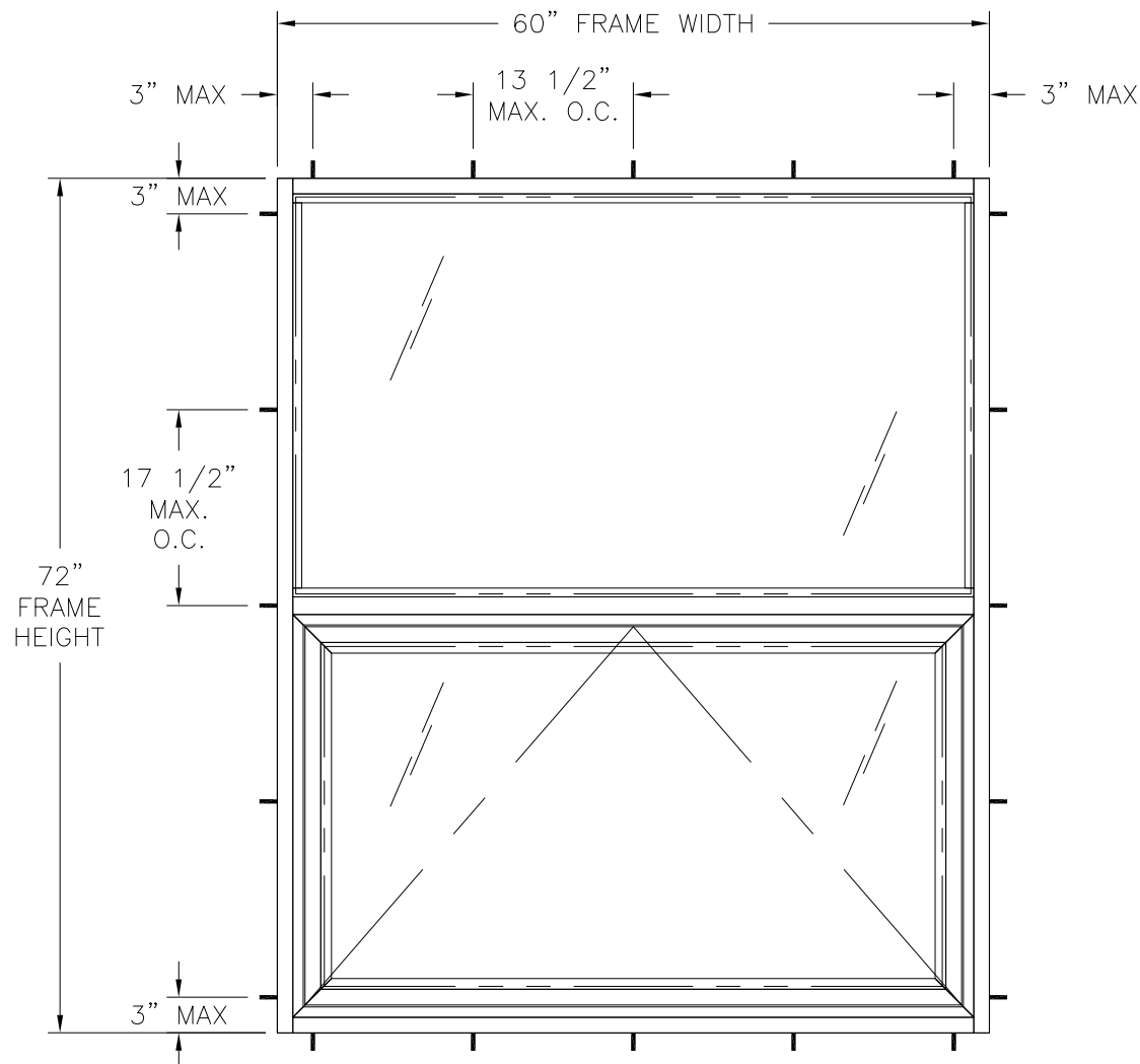
4300 SERIES FIXED PROJECT OUT WINDOW NON-IMPACT EXTERIOR VIEW
