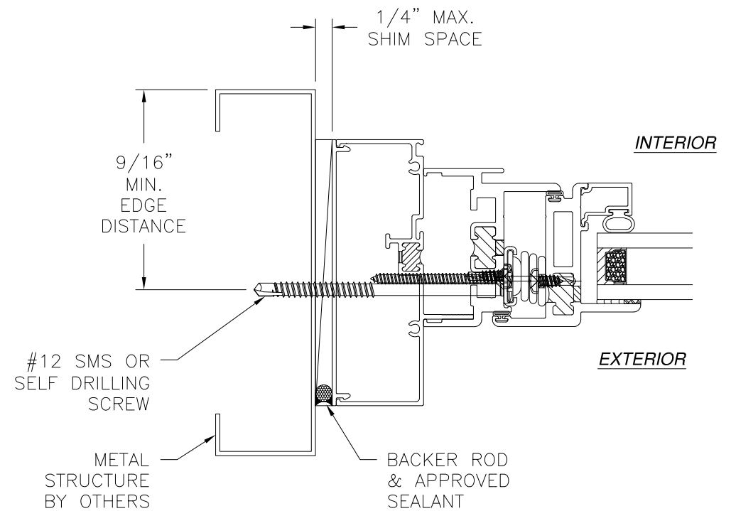
JAMB INSTALLATION DETAIL METAL STRUCTURE INSTALLATION PROJECT OUT WINDOW SHOWN
