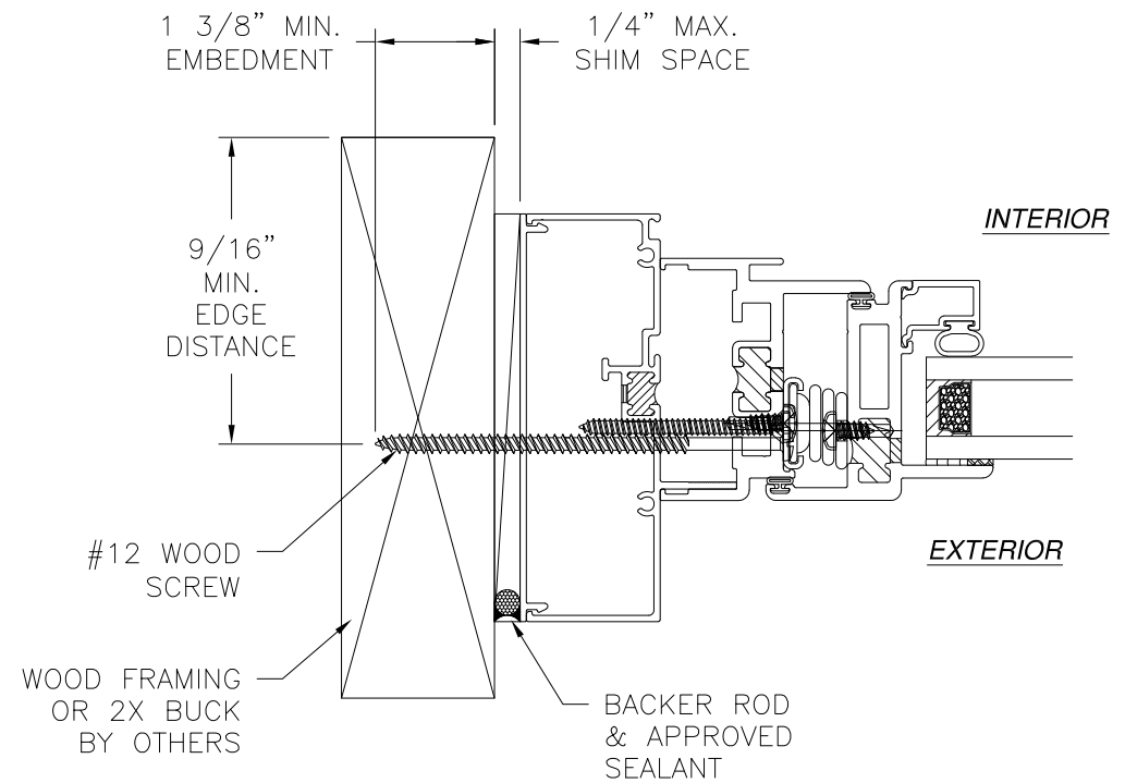
JAMB INSTALLATION DETAIL WOOD FRAMING OR 2X BUCK INSTALLATION PROJECT OUT WINDOW SHOWN
