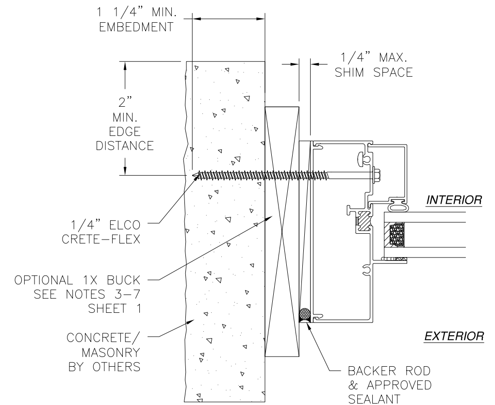
JAMB INSTALLATION DETAIL FIXED WINDOW CONCRETE/MASONRY WITH 1X BUCK INSTALLATION FOR INSTALLATION WITHOUT 1X BUCK REFER TO JAMB INSTALLATION DETAIL SHEET 5
