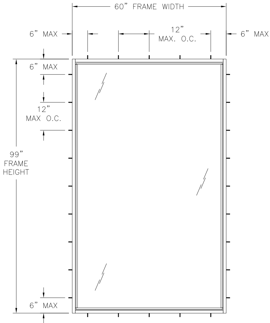
4000 SERIES FIXED WINDOW - IMPACT EXTERIOR VIEW
