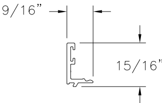
GLAZING BEAD (BAM-1015) ALUMINUM 6063-T6
