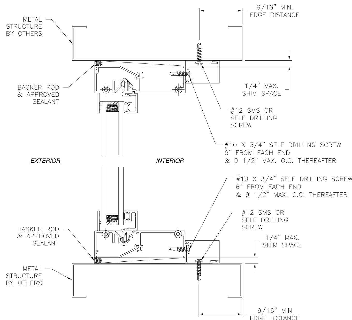
VERTICAL CROSS SECTION METAL STRUCTURE INSTALLATION
