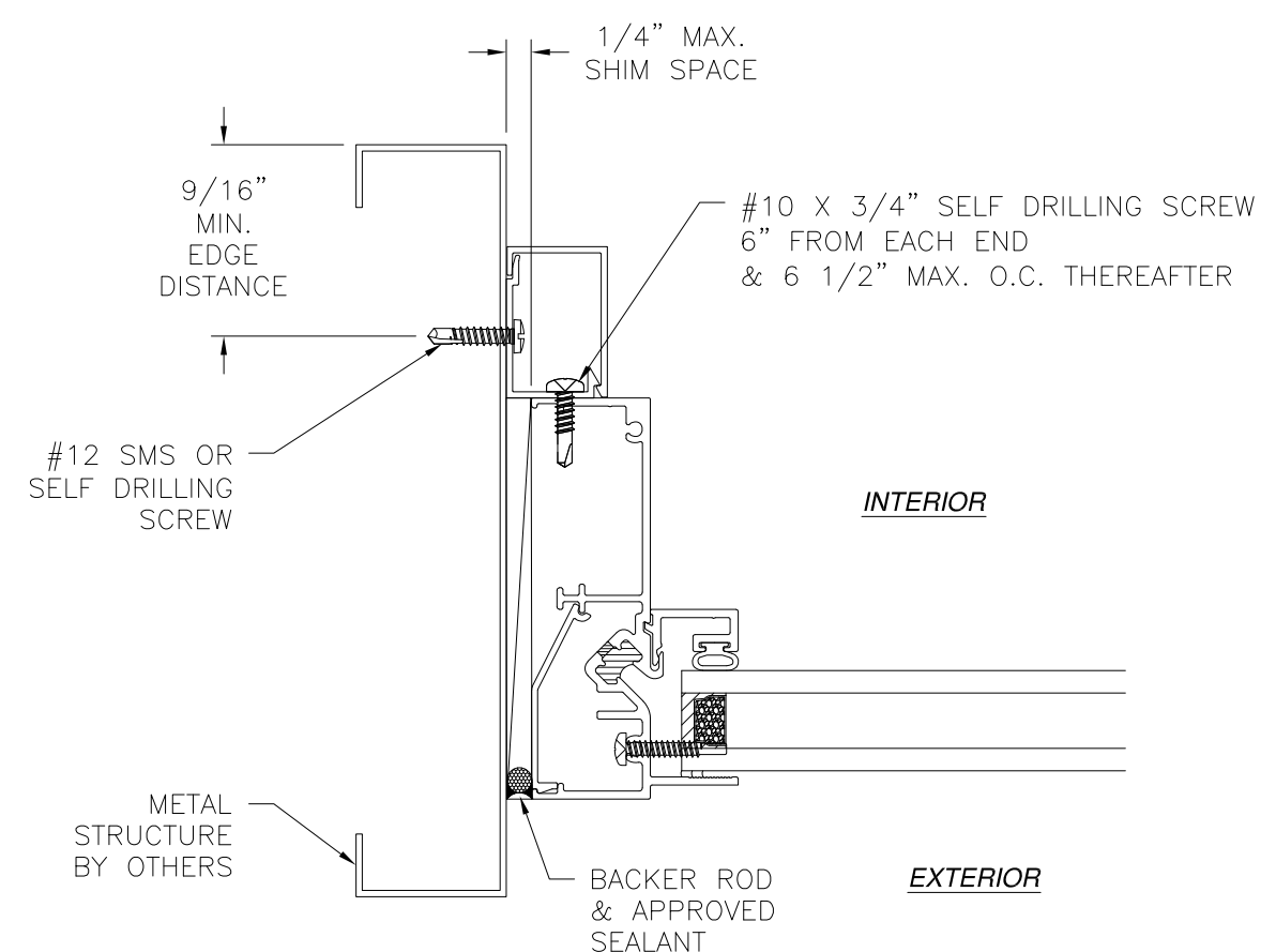
JAMB INSTALLATION DETAIL METAL STRUCTURE INSTALLATION
