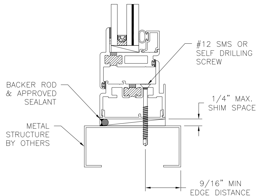
VERTICAL CROSS SECTION METAL STRUCTURE INSTALLATION
