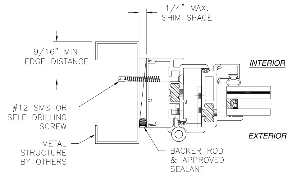
JAMB INSTALLATION DETAIL METAL STRUCTURE INSTALLATION CASEMENT WINDOW SHOWN
