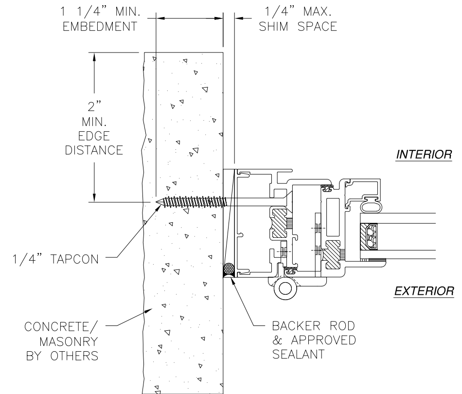
JAMB INSTALLATION DETAIL CONCRETE/MASONRY WITHOUT 1X BUCK INSTALLATION FOR CONCRETE/MASONRY WITH 1X BUCK REFER TO HEAD AND SILL INSTALLATION DETAILS CASEMENT WINDOW SHOWN
