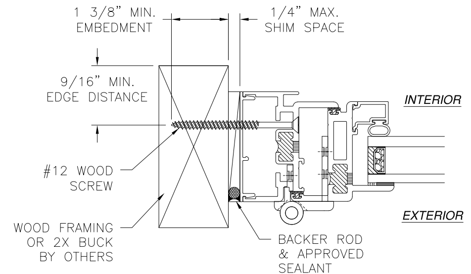
JAMB INSTALLATION DETAIL WOOD FRAMING OR 2X BUCK INSTALLATION CASEMENT WINDOW SHOWN
