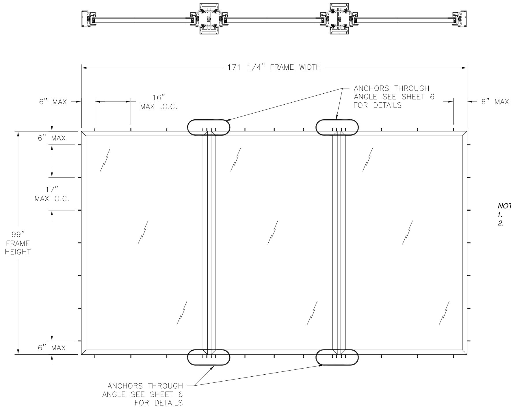
2200 SERIES TRIPLE FIXED WINDOW - IMPACT EXTERIOR VIEW
