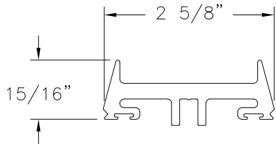
MULLION STIFFENER (BAM-1034) ALUMINUM 6063-T6
