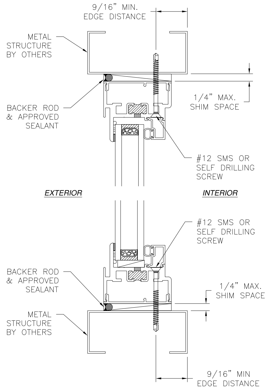
VERTICAL CROSS SECTION METAL STRUCTURE INSTALLATION
