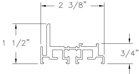
MAIN FRAME (BAM-911) ALUMINUM 6063-T5
