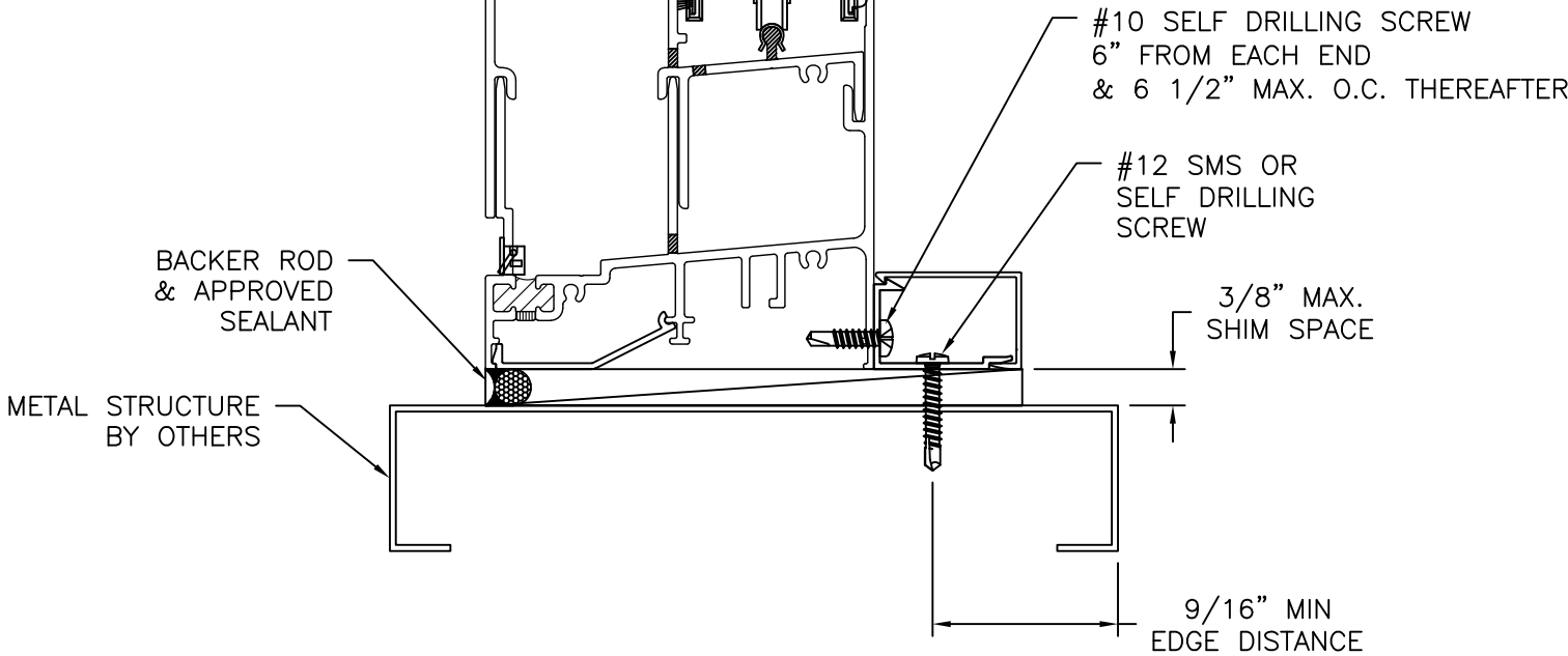
VERTICAL CROSS SECTION METAL STRUCTURE INSTALLATION
