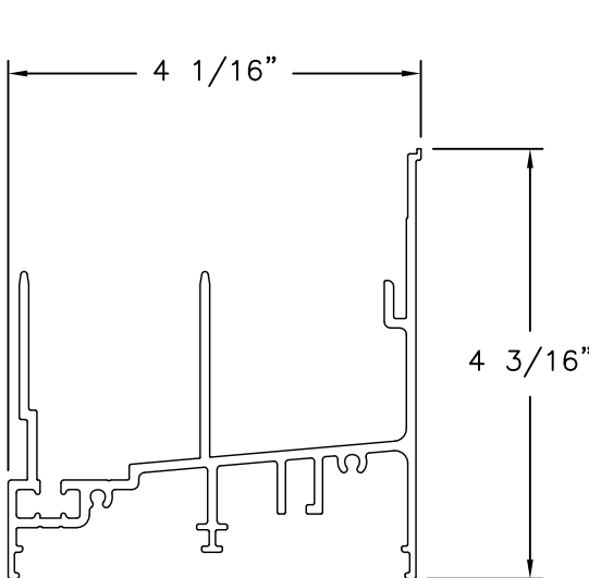
SILL (BAM-1201) ALUMINUM 6063-T6
