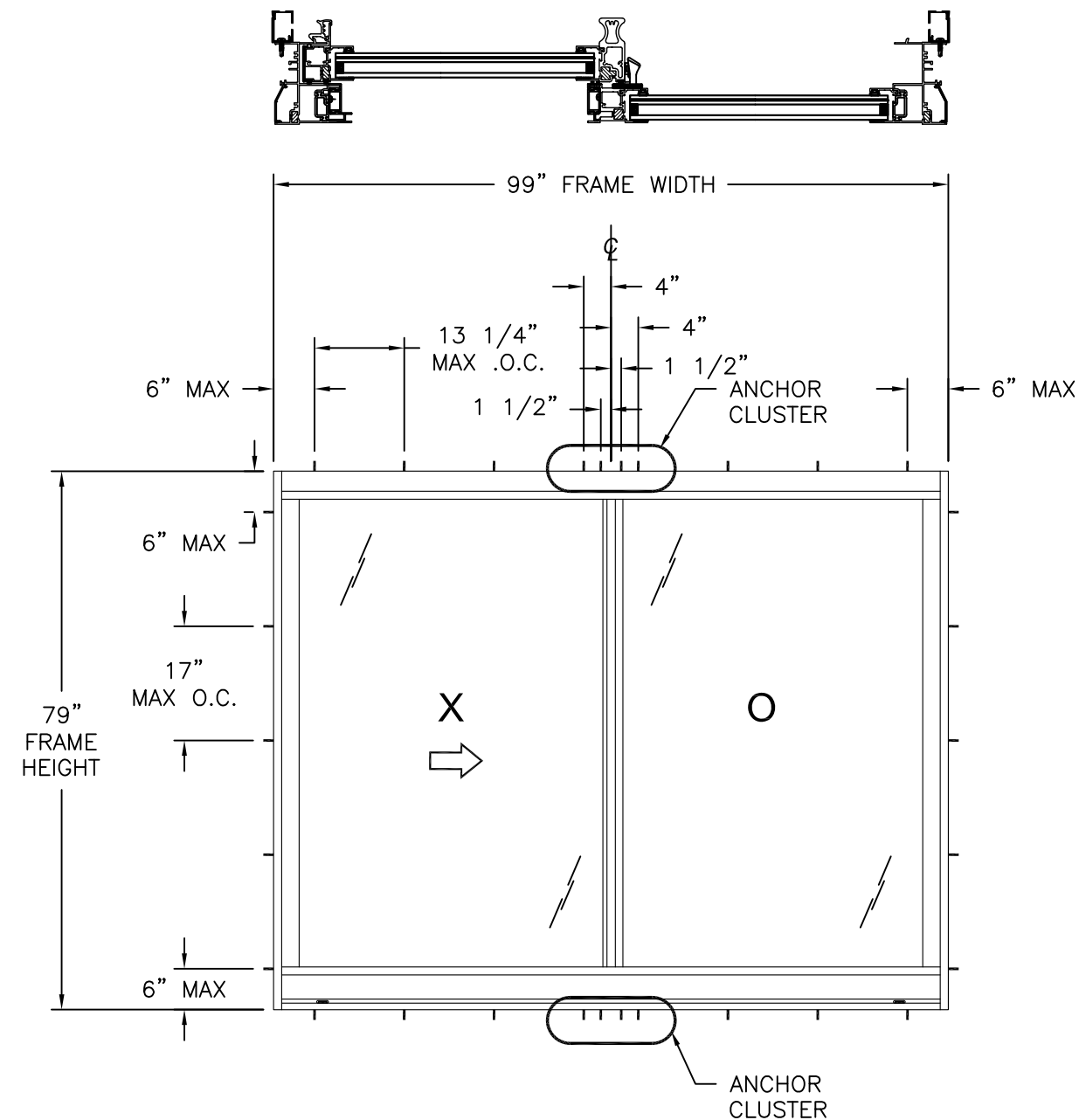
950 SERIES HORIZONTAL SLIDING WINDOW OX NON-IMPACT EXTERIOR VIEW
