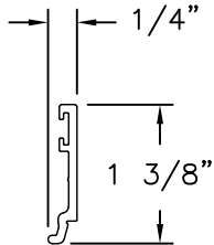
GLAZING BEAD (BAM-2015) ALUMINUM 6063-T6
