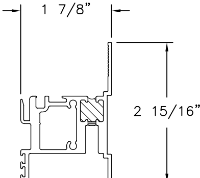
FIXED KEEPER RAIL (BAM-1205) ALUMINUM 6063-T5
