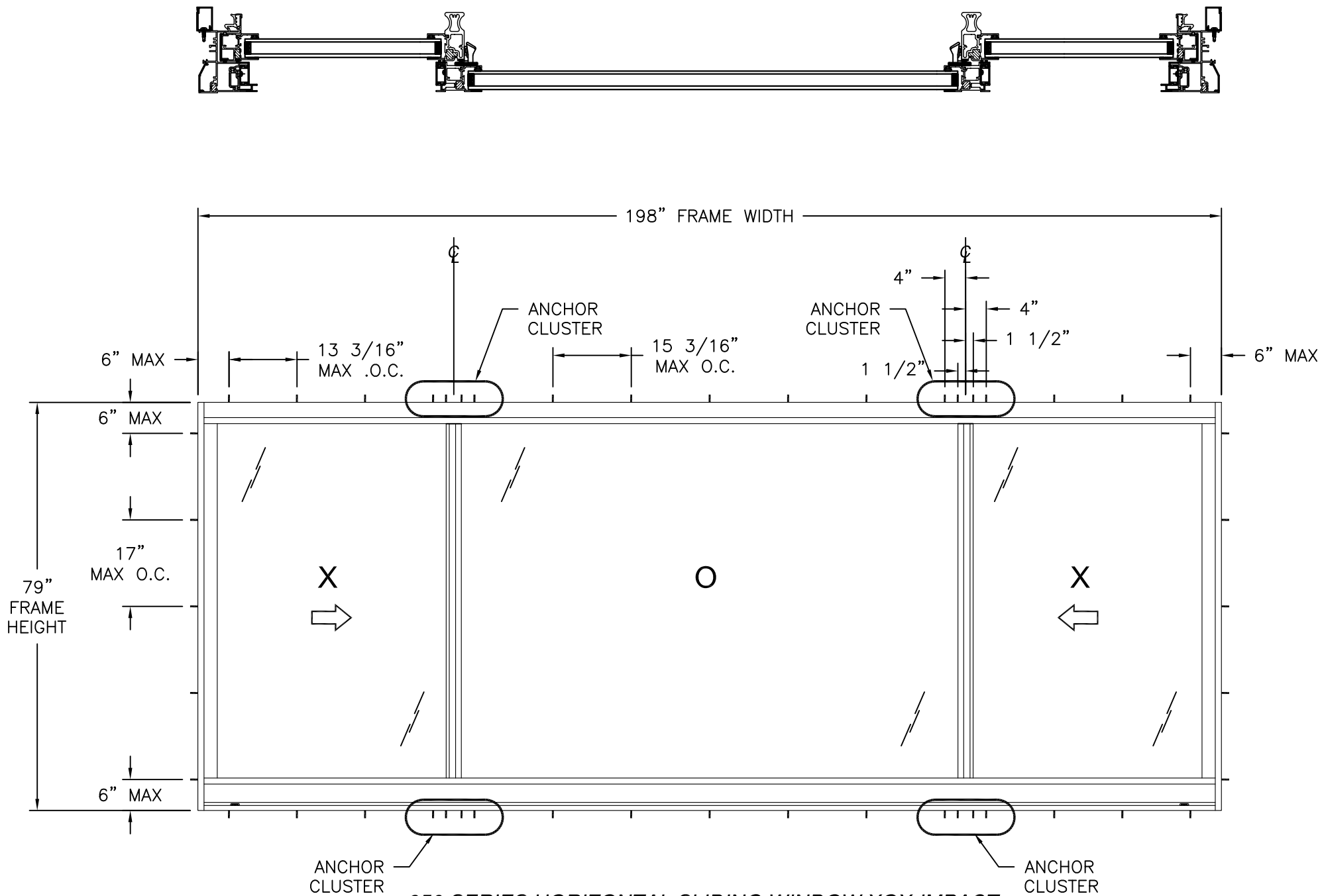
950 SERIES HORIZONTAL SLIDING WINDOW XOX-IMPACT EXTERIOR VIEW
