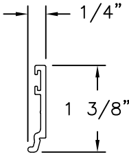
GLAZING BEAD (BAM-2015) ALUMINUM 6063-T6
