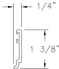
GLAZING BEAD (BAM-2015) ALUMINUM 6063-T6
