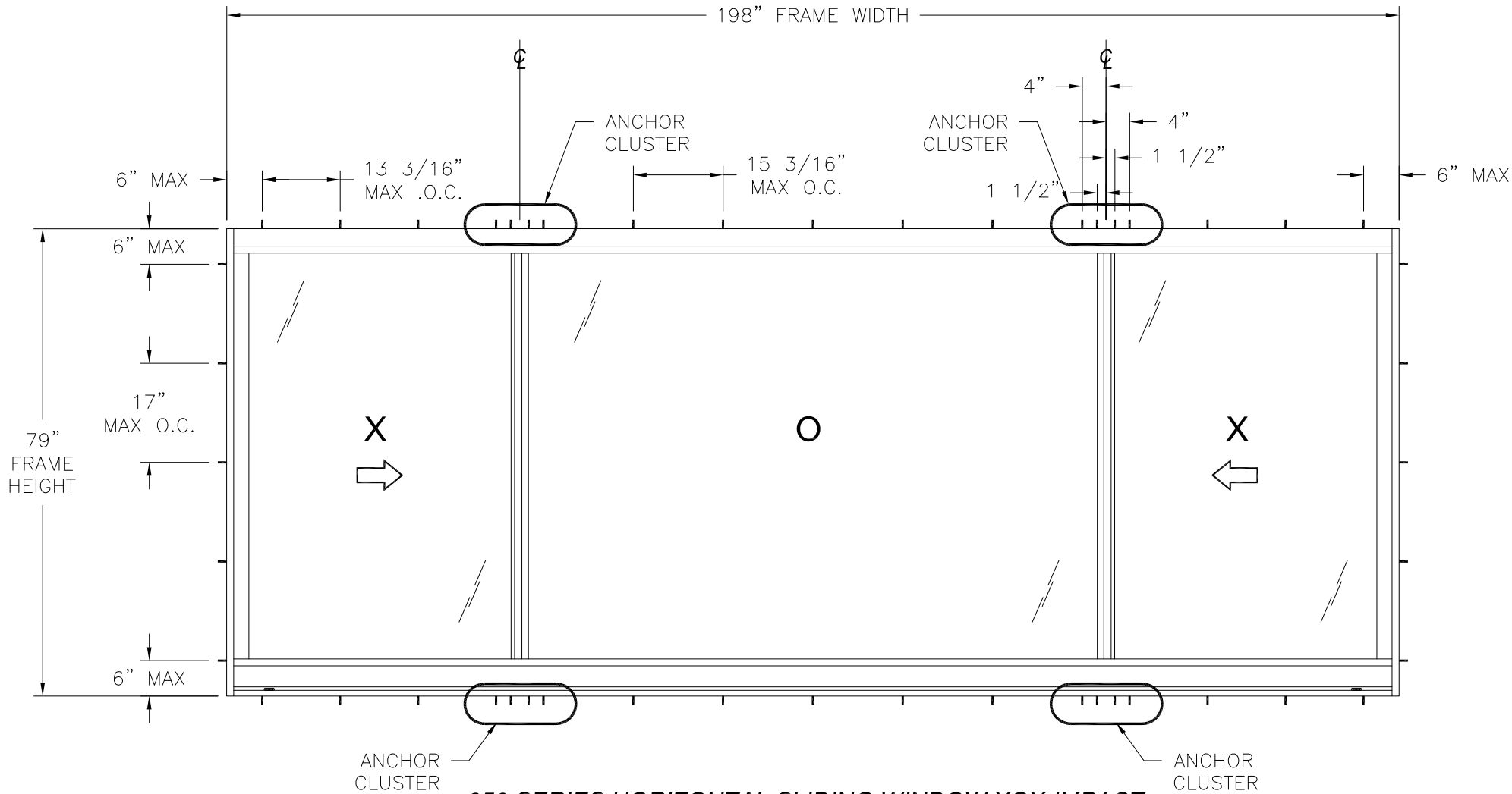
950 SERIES HORIZONTAL SLIDING WINDOW XOX-IMPACT EXTERIOR VIEW
