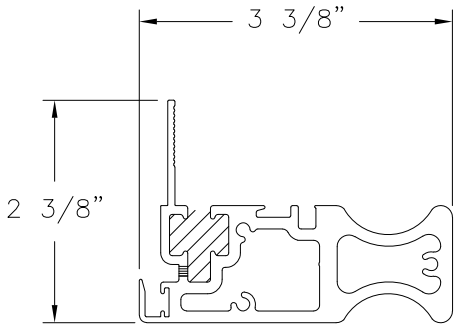
LOCK RAIL (BAM-1207) ALUMINUM 6063-T5
