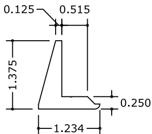
11 SILL ANCHOR
