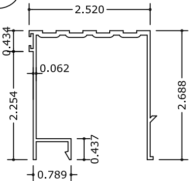
12 THRESHOLD FILLING TRACK
