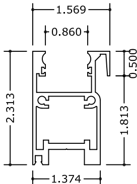
8 OUTSIDE BOTTOM RAIL
