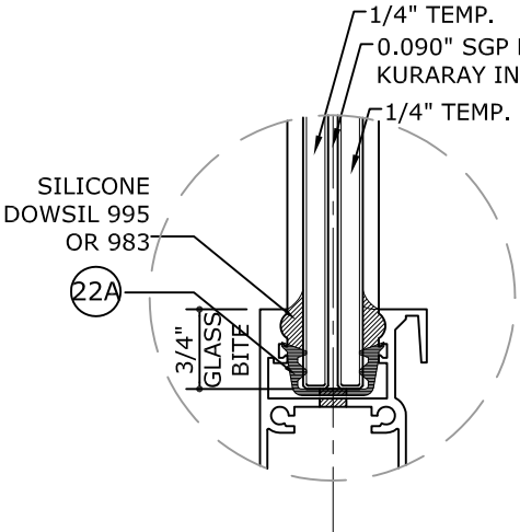
GLAZING DETAIL - GLASS TYPE '1' SMALL MISSILE IMPACT
