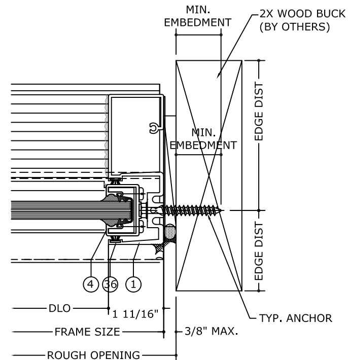
3.4 FIXED JAMB DETAIL (WOOD) N.T.S.
