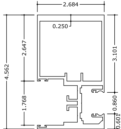
5 MEETING STILE
