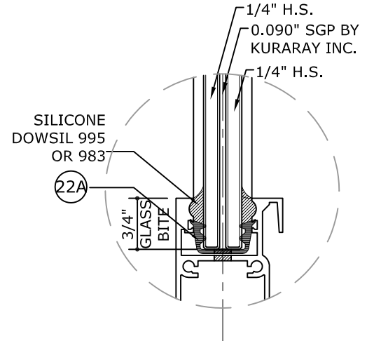
GLAZING DETAIL - GLASS TYPE '3' LARGE MISSILE IMPACT- LEVEL D
