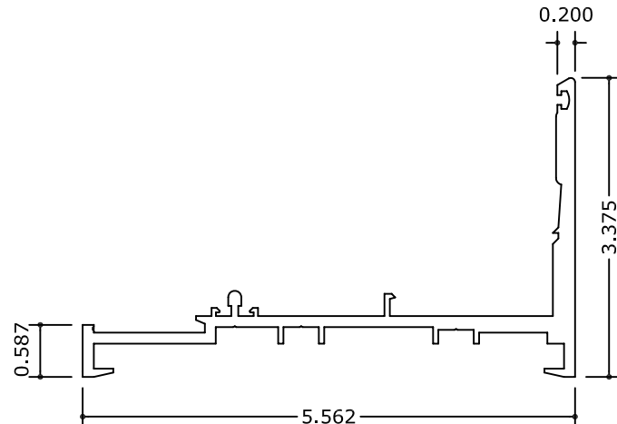
10 SILL TRACK
