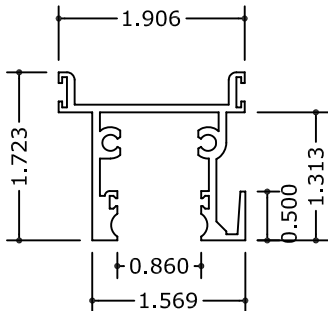
6 OUTSIDE TOP RAIL
