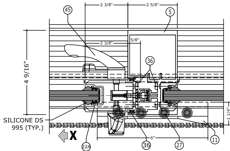
6 MEETING STILES DETAIL N.T.S
