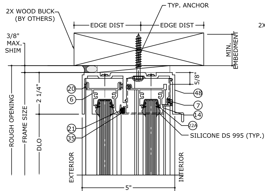
1.2A HEAD DETAIL (WOOD) N.T.S.
