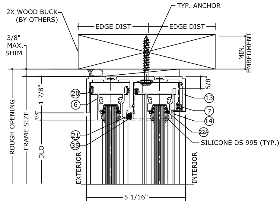
1.2 HEAD DETAIL (WOOD) N.T.S.
