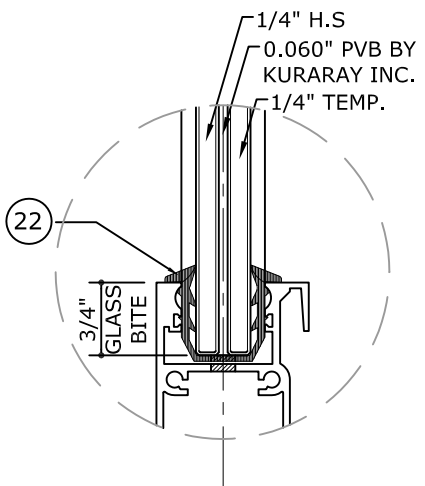
GLAZING DETAIL - GLASS TYPE '1A' SMALL MISSILE IMPACT
