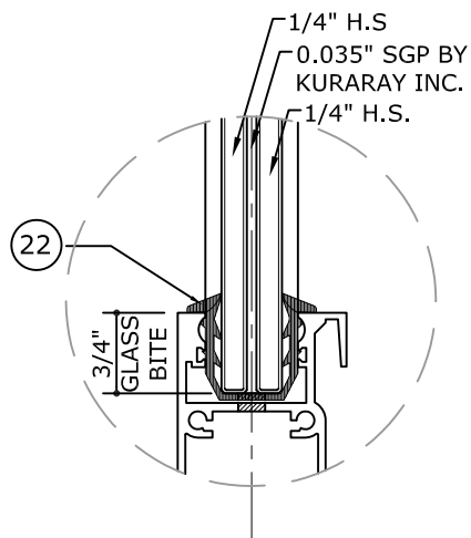
GLAZING DETAIL - GLASS TYPE '2' SMALL MISSILE IMPACT
