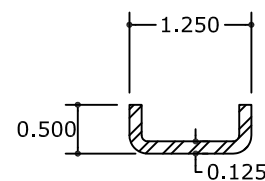
51 S.S. REINFORCEMENT CHANNEL
