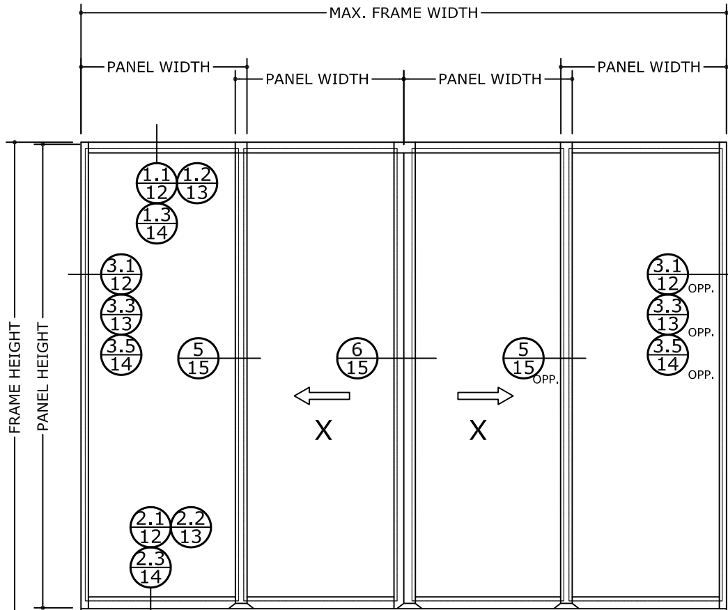
TYPICAL ELEVATION LOOKING FROM OUTSIDE IN
