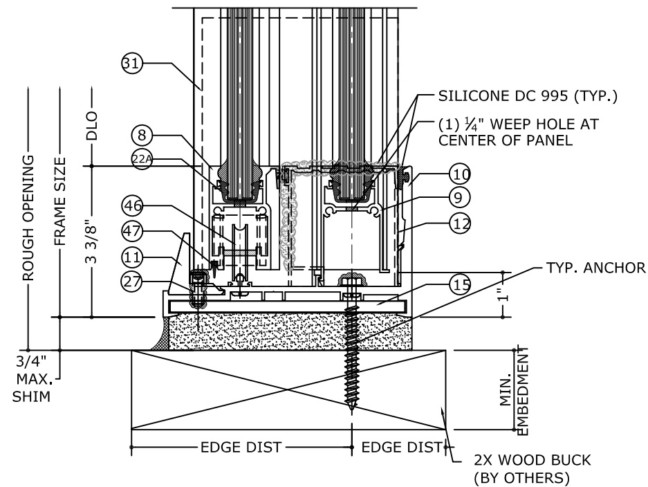
2.2 SILL DETAIL (WOOD) N.T.S.
