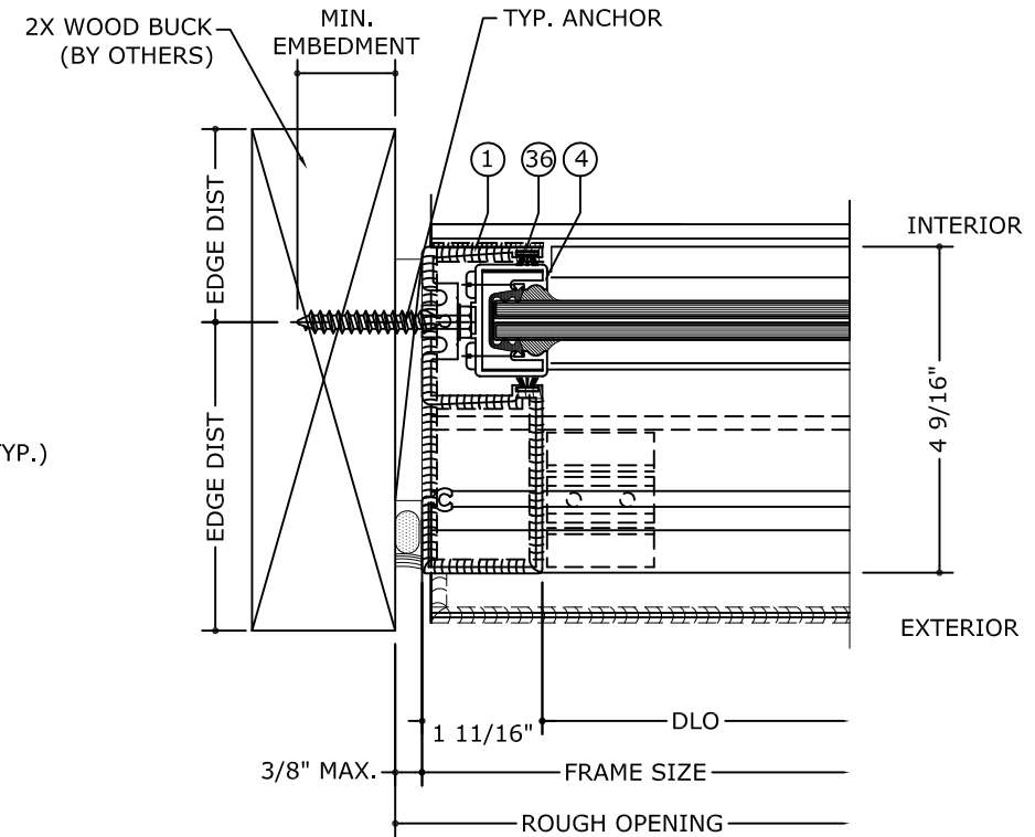
3.3 FIXED JAMB DETAIL (WOOD) N.T.S.
