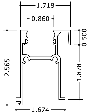
9 INSIDE BOTTOM RAIL
