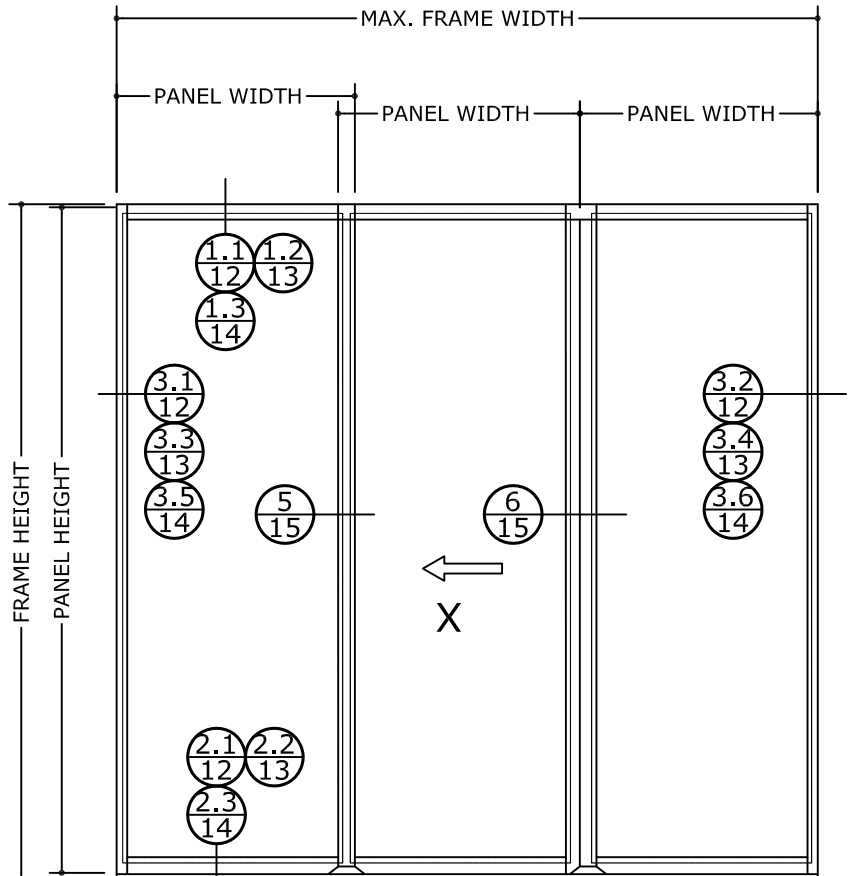
TYPICAL ELEVATION LOOKING FROM OUTSIDE IN
