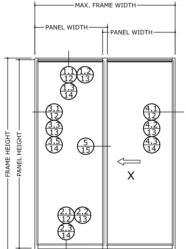
TYPICAL ELEVATION LOOKING FROM OUTSIDE IN
