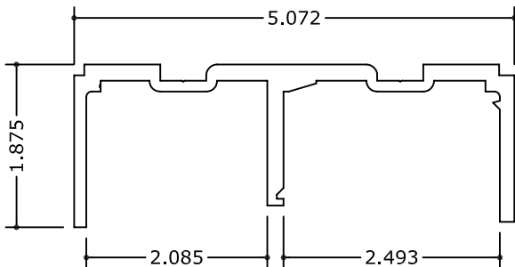
13 HEAD TRACK
