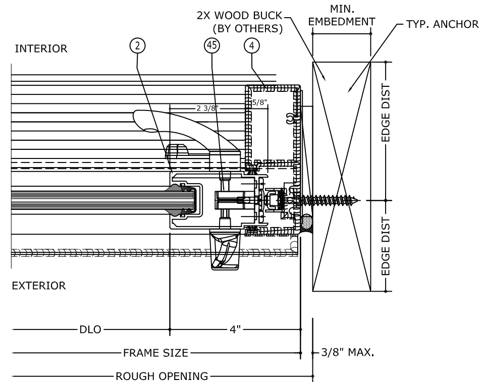
4.2 OPERABLE JAMB DETAIL (WOOD) N.T.S.
