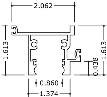
7 INSIDE TOP RAIL
