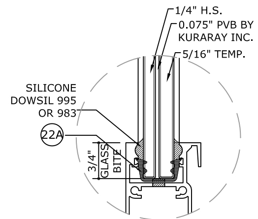
GLAZING DETAIL - GLASS TYPE '4' SMALL MISSILE IMPACT
