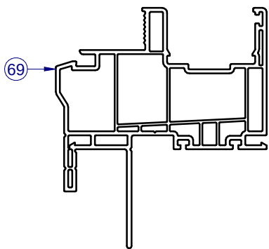
SECTION C-C ALTERNATE FRAME FLANGE WITH FIN
