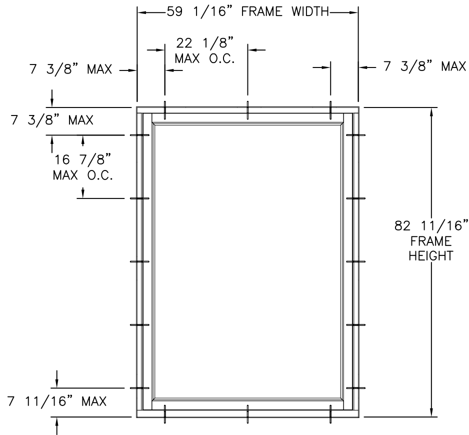
SINGLE RECTANGULAR FIXED WINDOW INTERIOR VIEW
