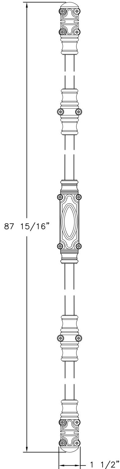
CREMONE TYPE RG 50 FROM REMY GARNIER
