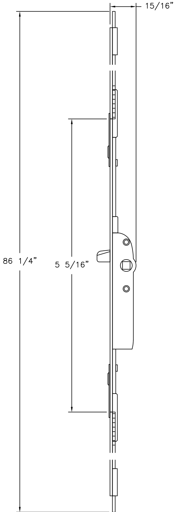
3 POINT MORTISE CREMONE BOLT TYPE F 15 FROM FERCO
