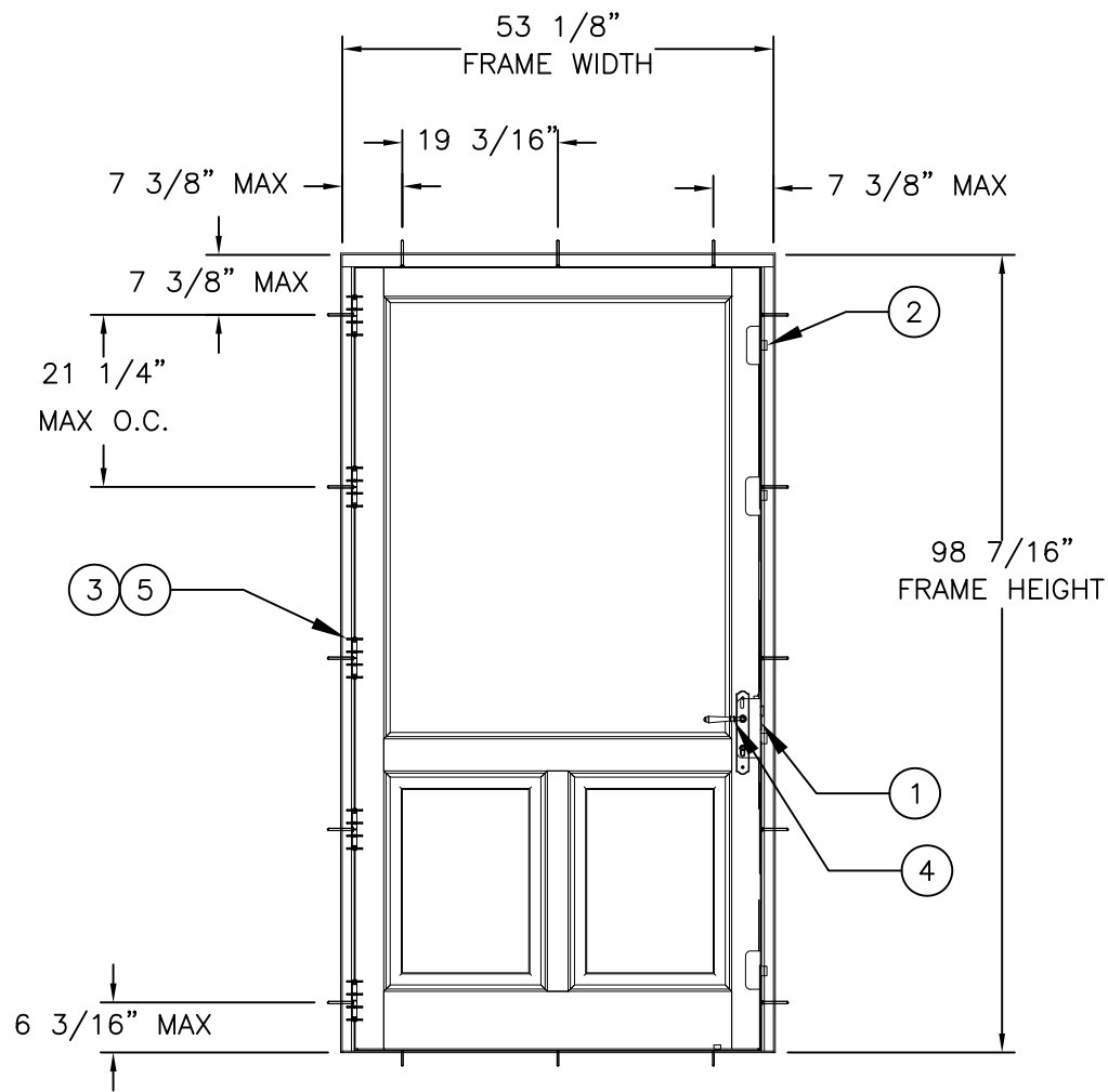
SINGLE RECTANGULAR DOOR INTERIOR VIEW
