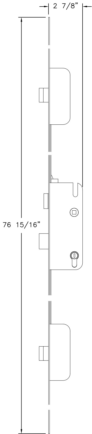
3 POINT LOCK TYPE SF2 FROM G.U-SECURY
