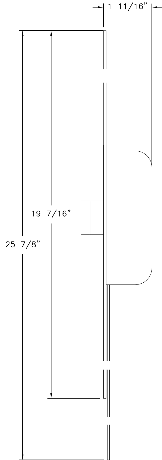
ADDITIONAL LOCK TYPE SF FROM G.U-SECURY
