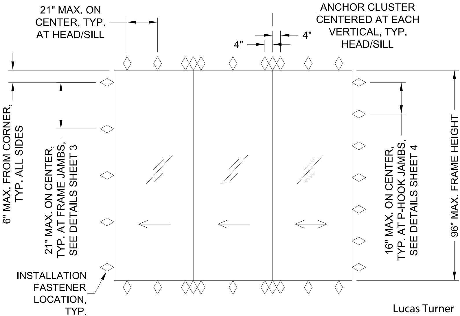
SAMPLE ELEVATION
