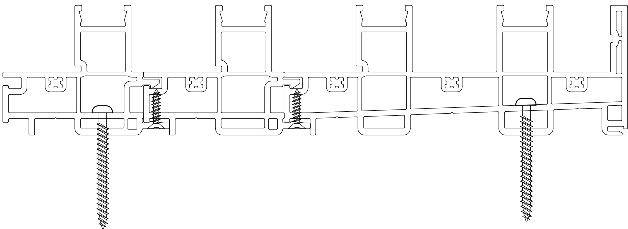
TYPICAL 4-TRACK FRAME ANCHOR LOCATIONS
