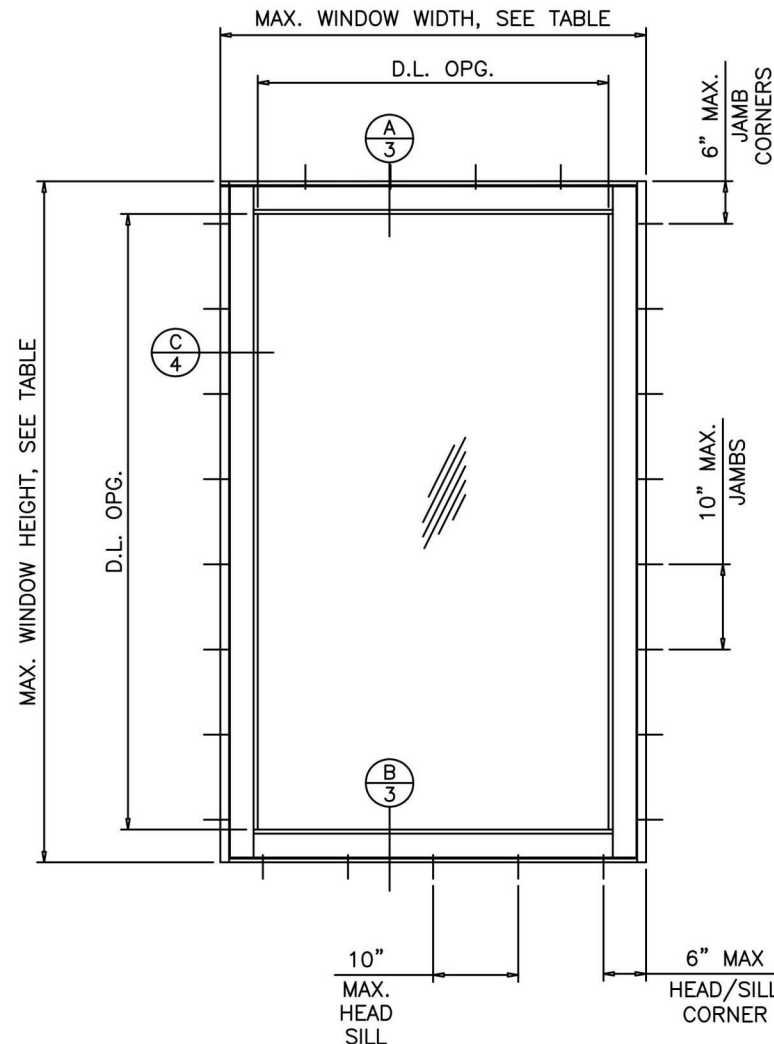
TYPICAL ELEVATION
