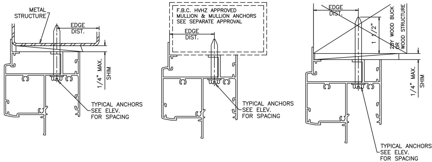
TYPICAL ANCHORS: SEE ELEV. FOR SPACING
