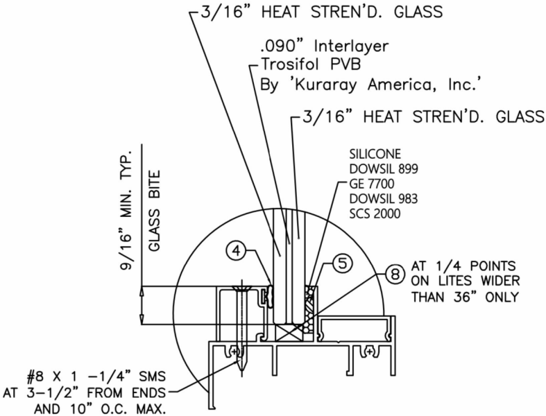
GLAZING DETAIL 7/16" OVERALL NOM. THK.
