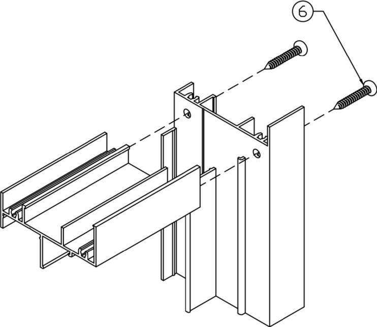
CORNER DETAIL
