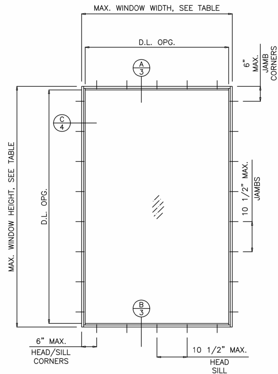
TYPICAL ELEVATION
