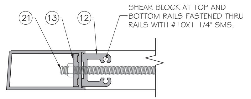
SECTION THRU RAILS
