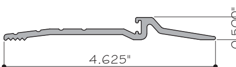
7 DOOR THRESHOLD WW520B (6063-T5)
