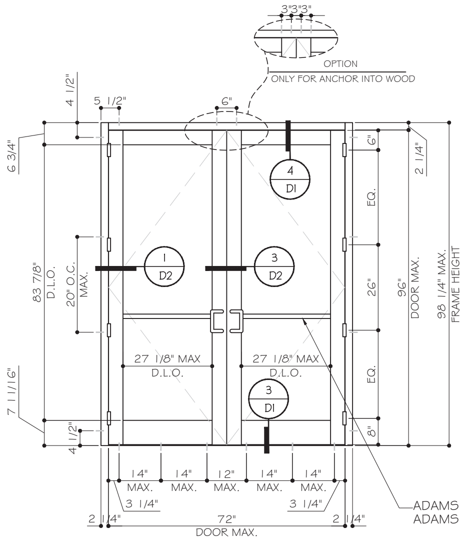
TYPICAL ELEVATIONS
