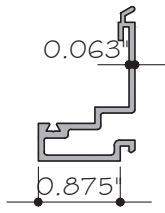
5 EXTER. GLASS STOP WW185 (6063-T5)
