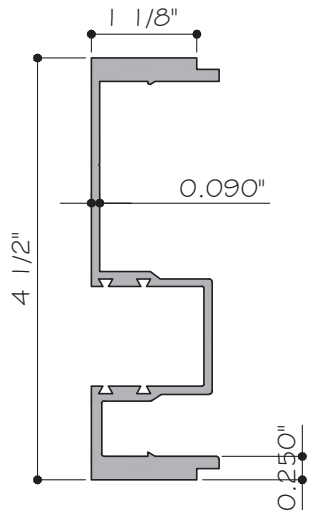
3 FRAME /JAMB BASE WW11M (6063-T5)
