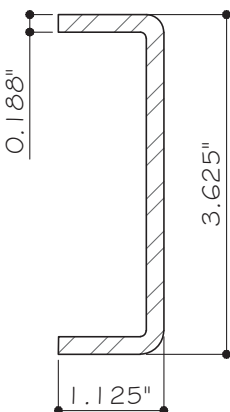
14 REINF. CHANNEL STEEL, 3 5/8"X1 1/8"X 3/16" THK.
