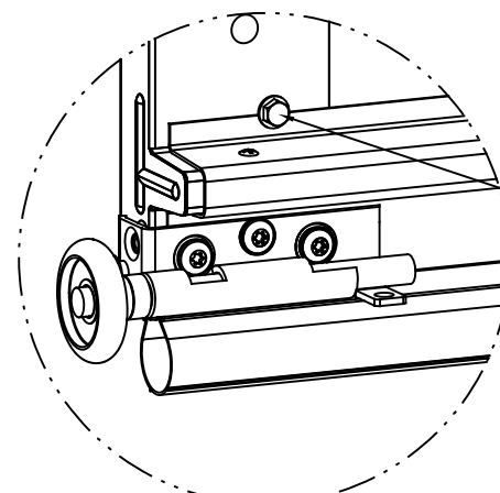
DETAIL D
