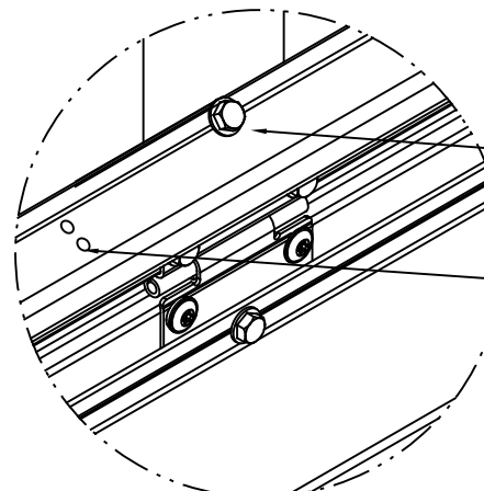
J-STRUT ATTACHMENT
