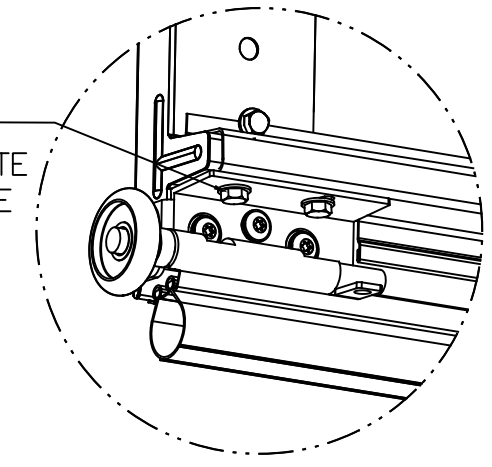
DETAIL D IMPACT BOTTOM BRACKET
