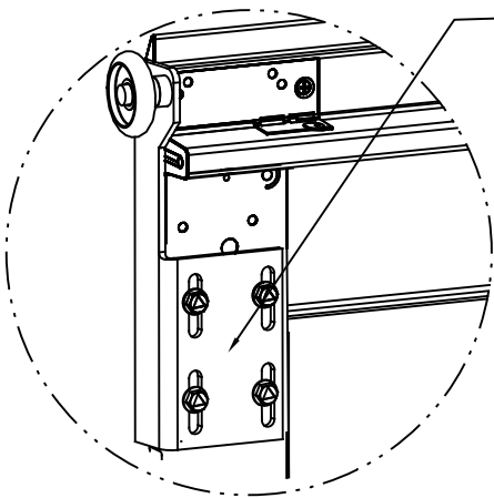
LOW HEADROOM TRACK
