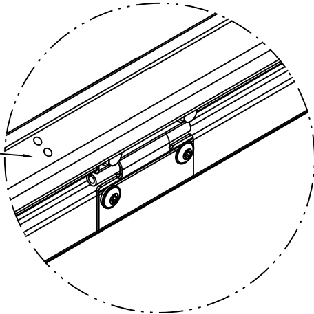
J-STRUT ATTACHMENT
