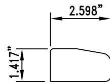
6 GLAZING STOP Scale: 1/2 FULL SIZE
