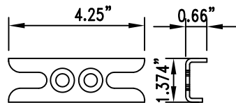
21 CAM KEEPER Scale: 1/2 FULL SIZE
