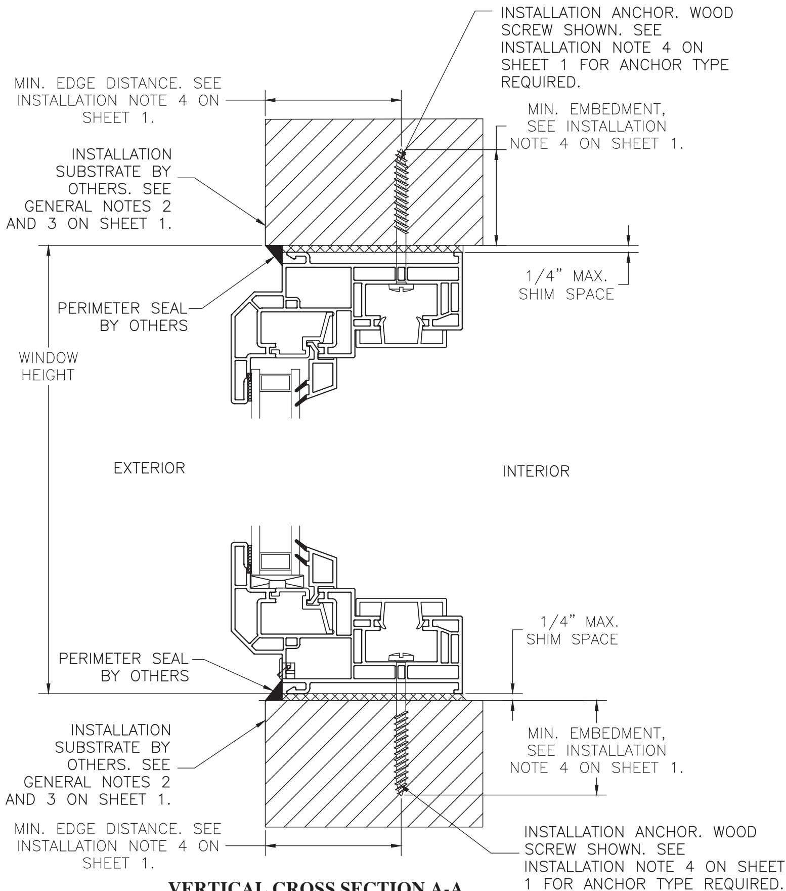
VERTICAL CROSS SECTION A-A WOOD FRAMING, 2X WOOD BUCK, CONCRETE/MASONRY OR METAL FRAME APPROVED
