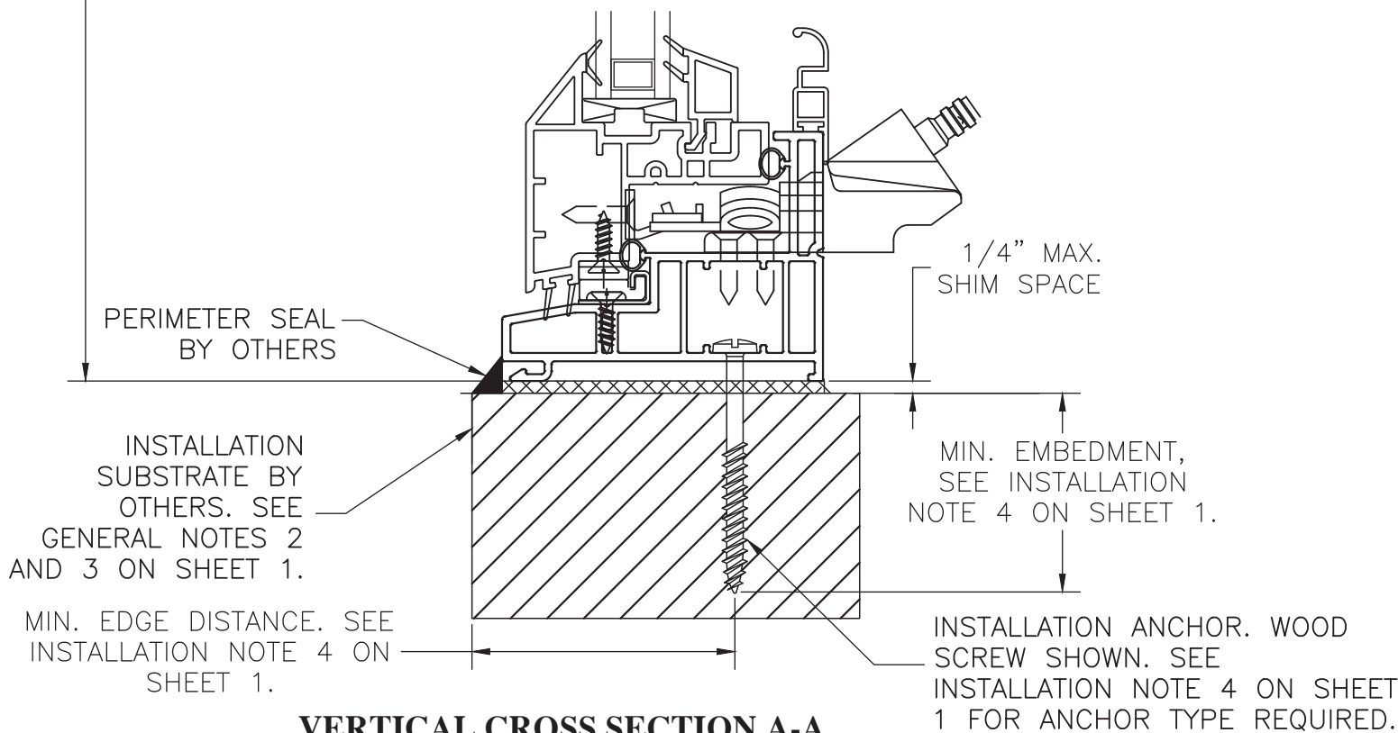
VERTICAL CROSS SECTION A-A WOOD FRAMING, 2X WOOD BUCK, CONCRETE/MASONRY OR METAL FRAME APPROVED
